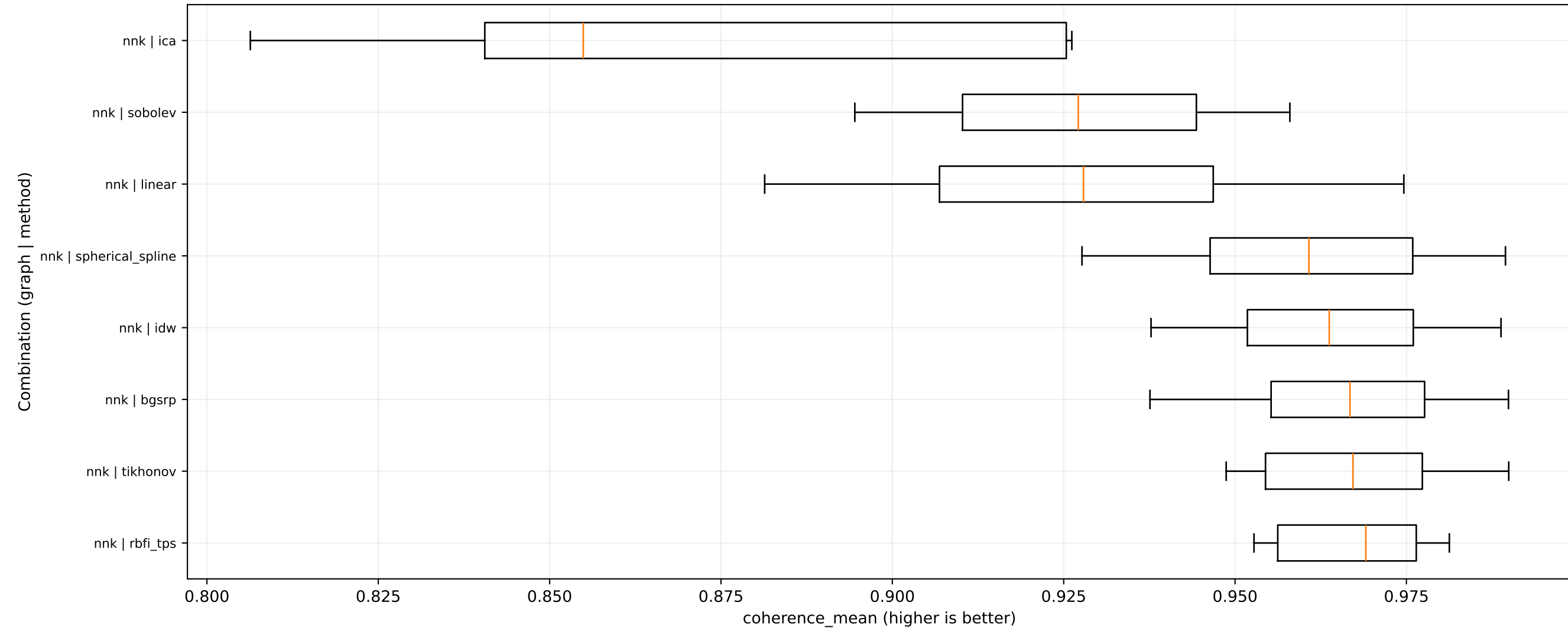
coherence_mean distribution by graph-method combination - dataset: physionet_eegmmidb_real
