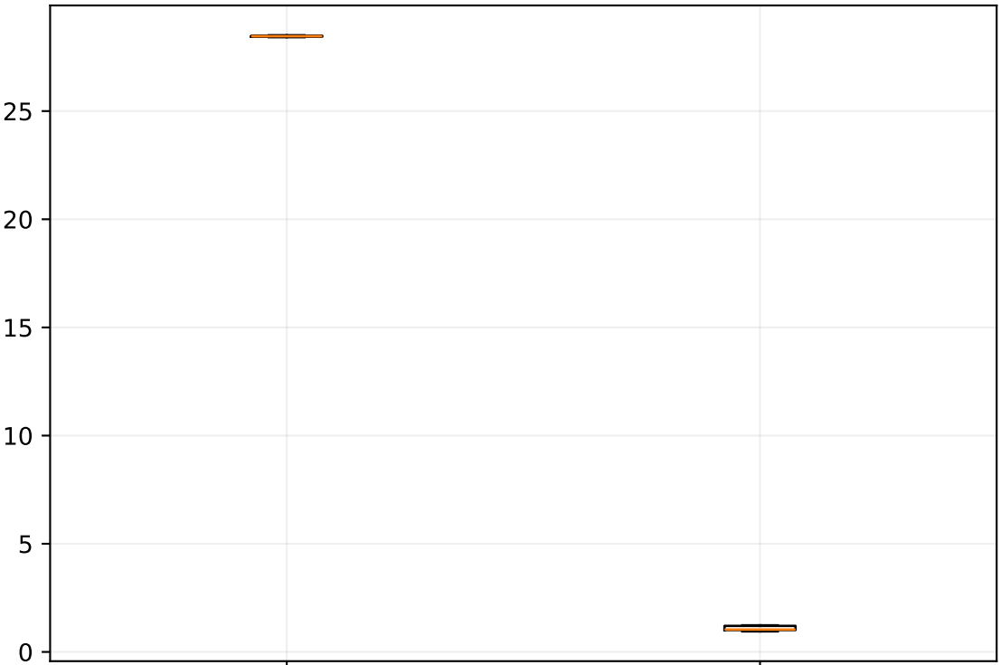
DTW
