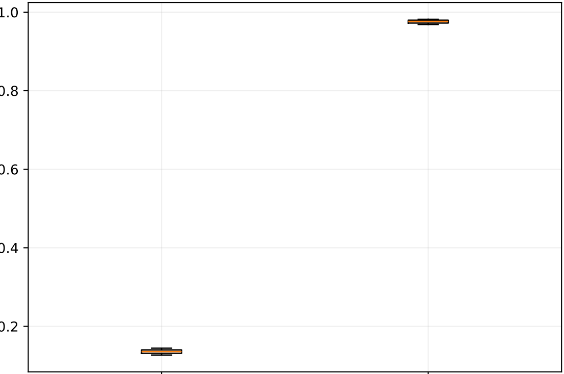
coherence_mean
