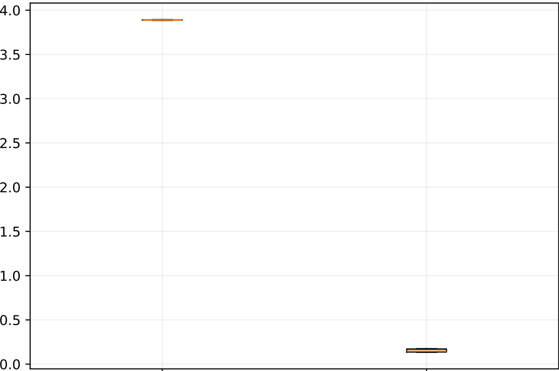
RMSE
