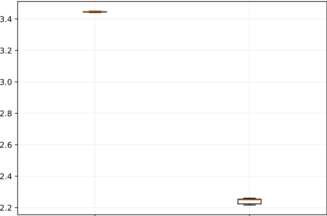
LSD
