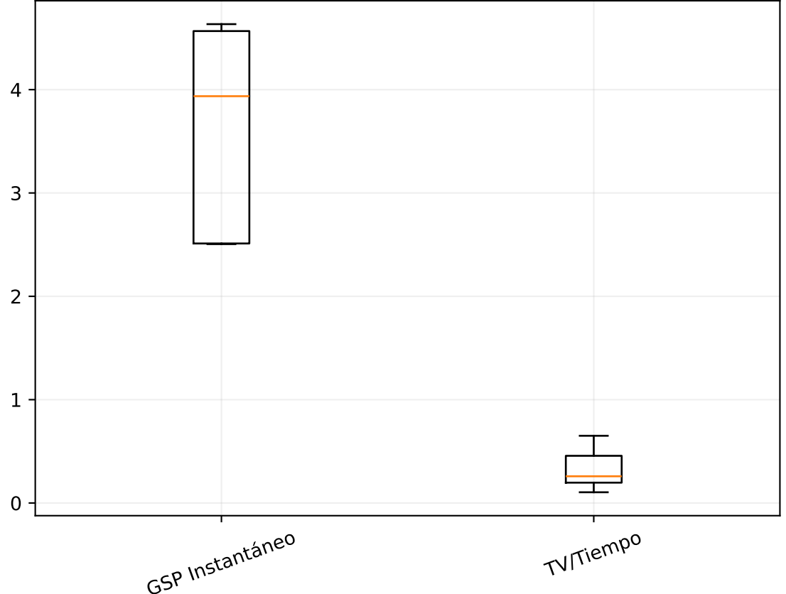
RMSE
