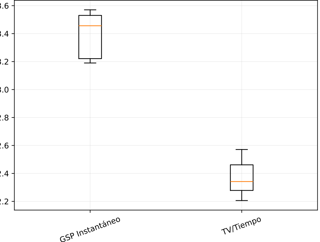
LSD
