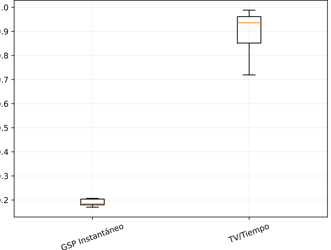
coherence_mean
