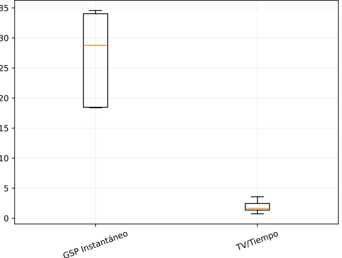
DTW
