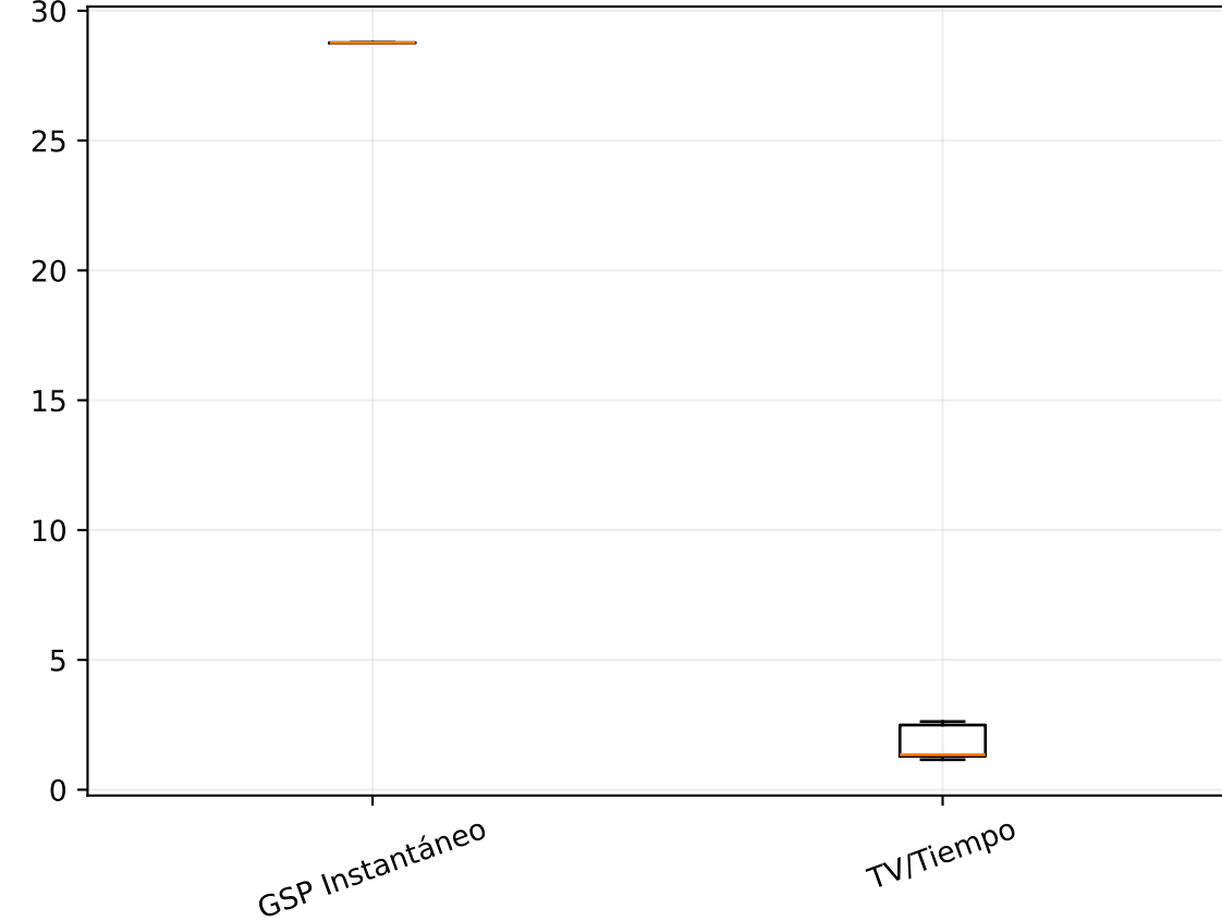
DTW
