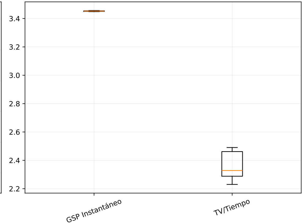
LSD
