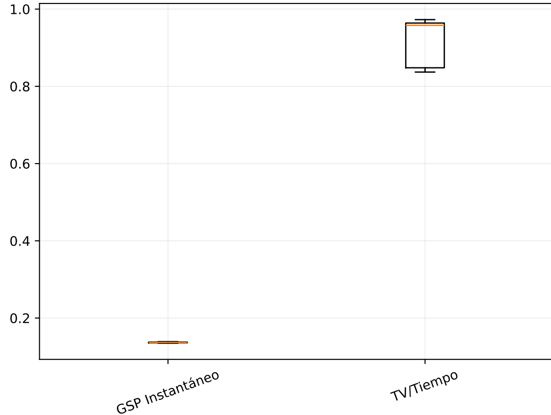
coherence_mean
