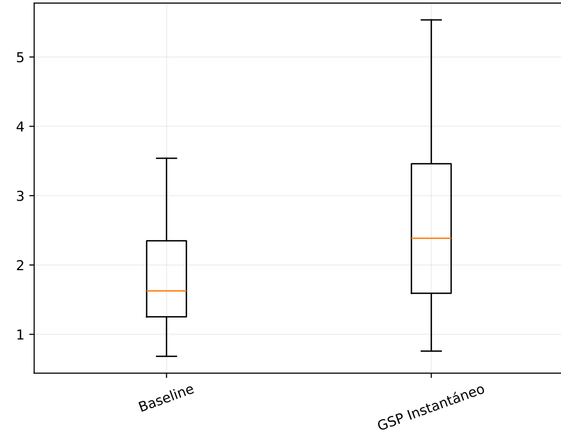
DTW
