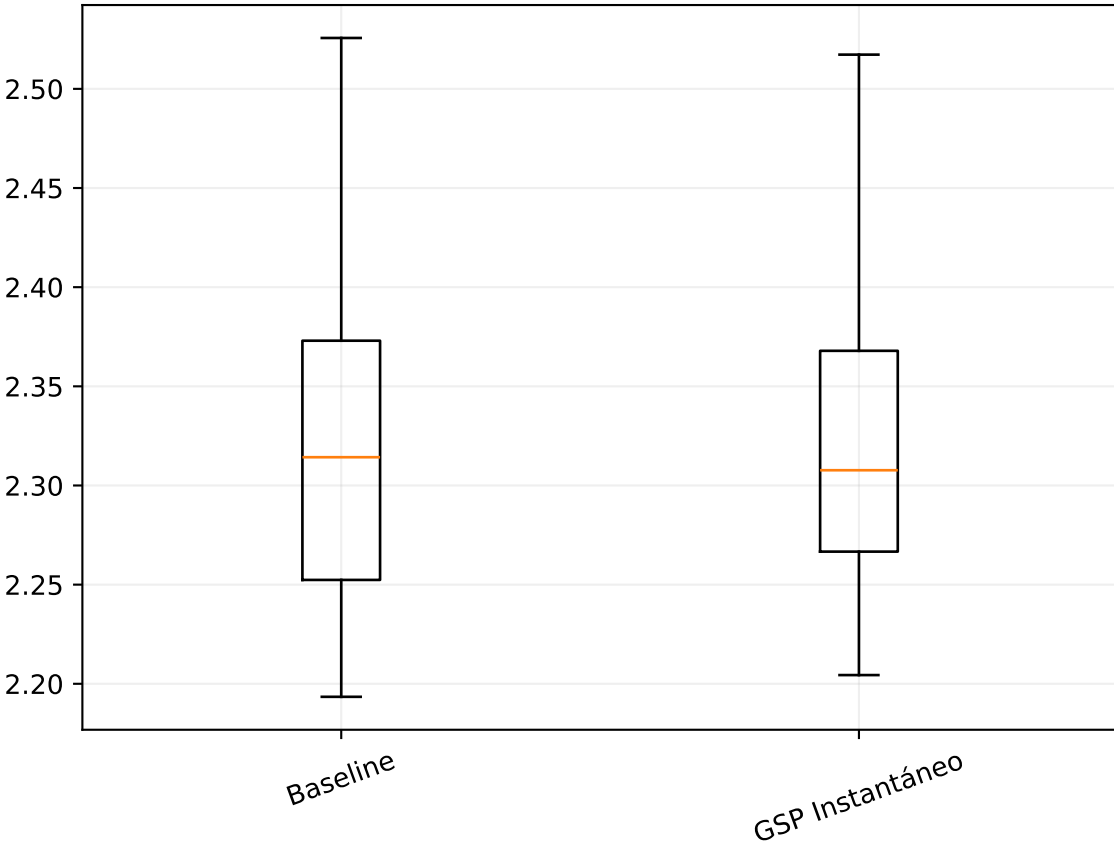
LSD
