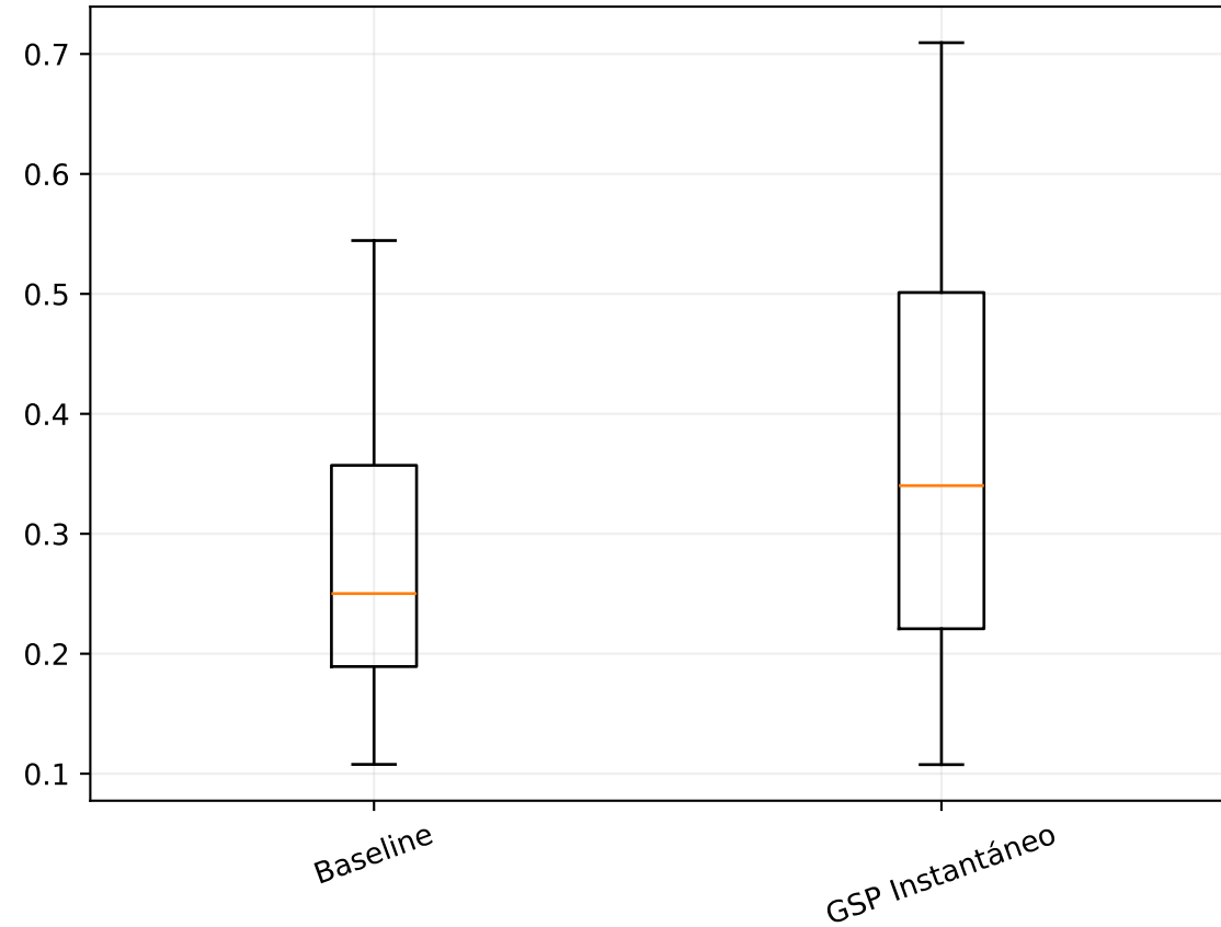
RMSE
