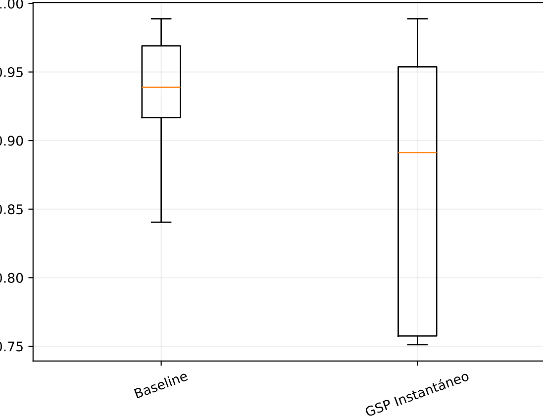
coherence_mean
