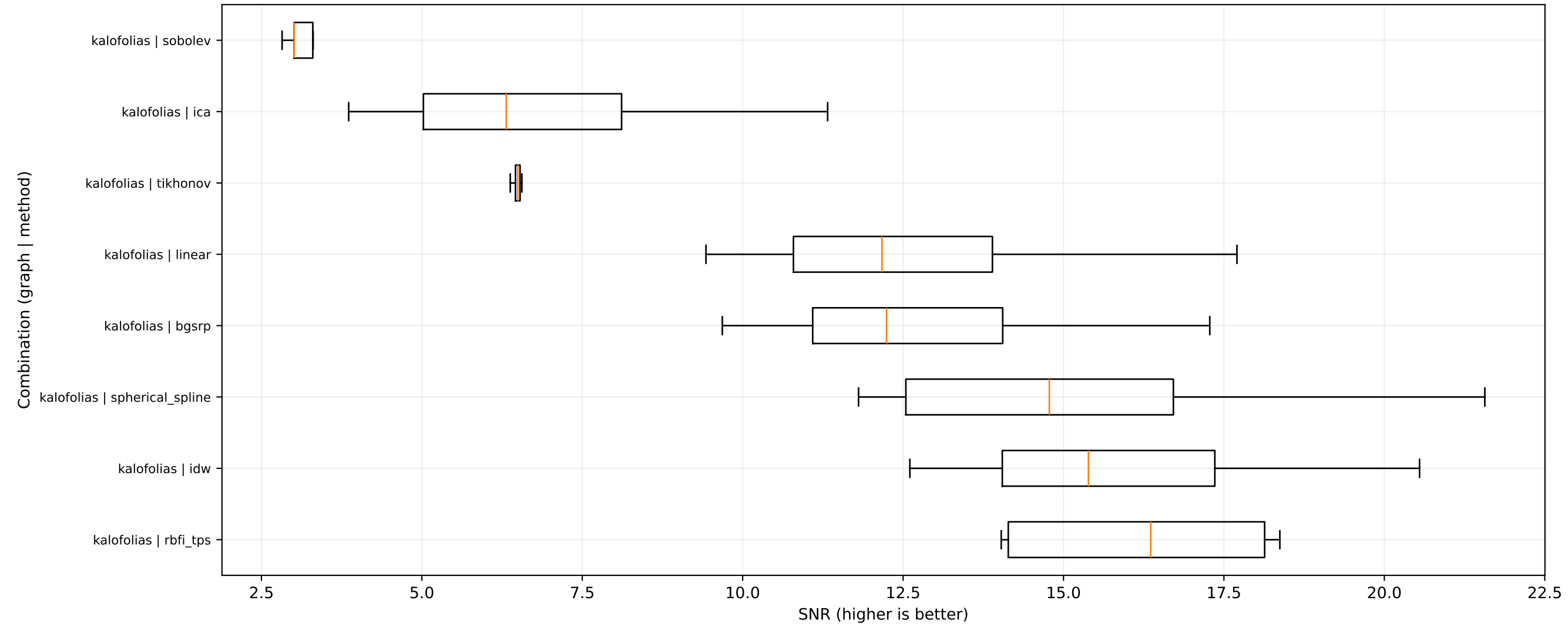
SNR distribution by graph-method combination - dataset: physionet_eegmmbd_real
