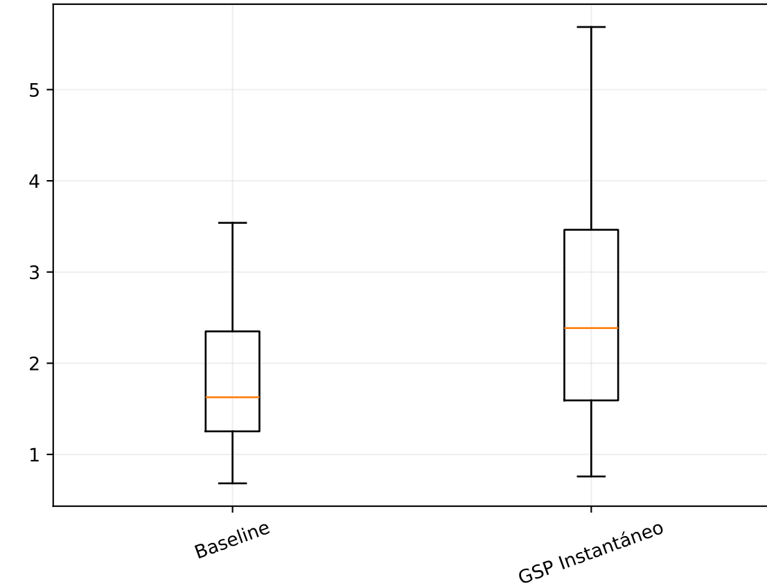
DTW
