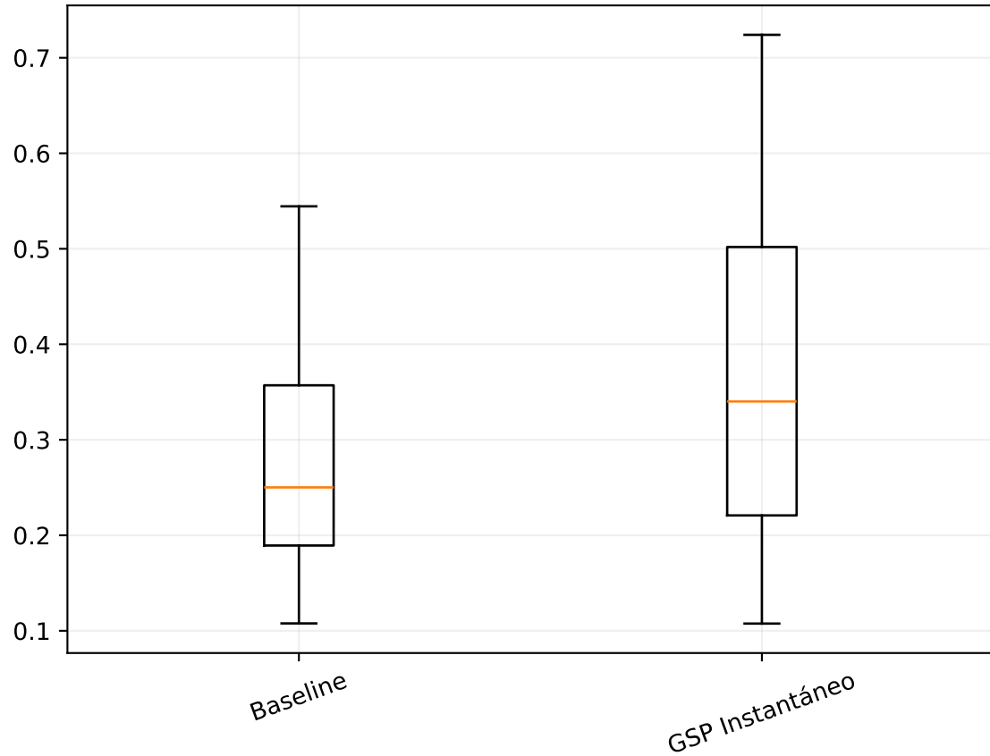
RMSE
