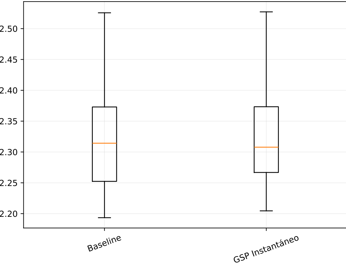
LSD
