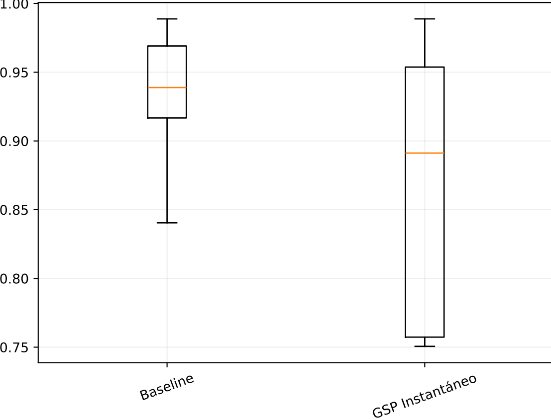
coherence_mean
