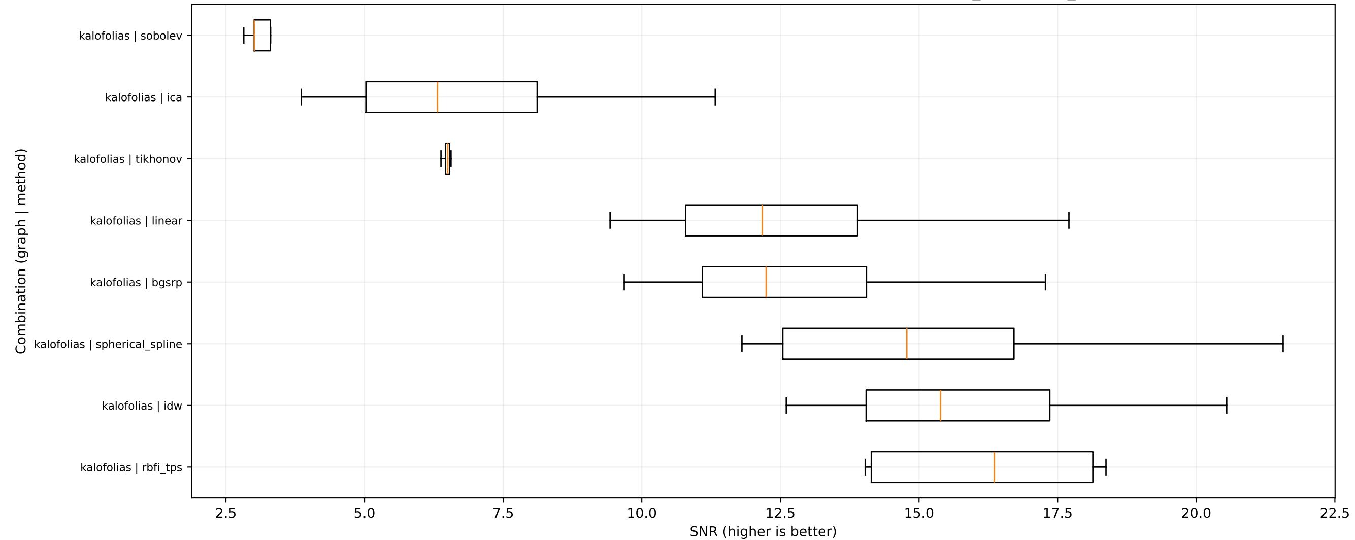
SNR distribution by graph-method combination - dataset: physionet_eegmmb_real
