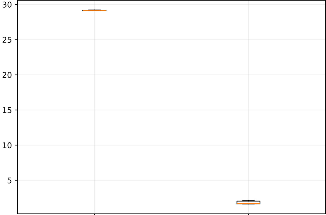
DTW
