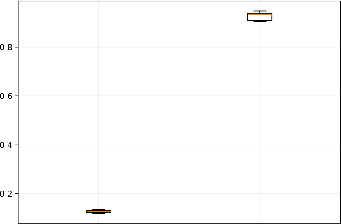
coherence_mean
