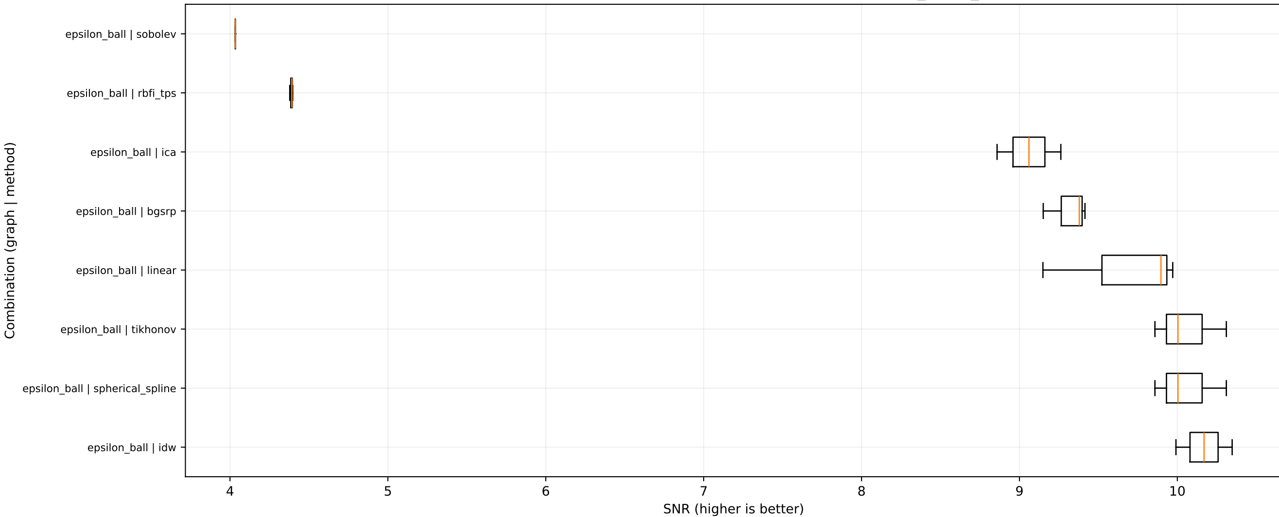
SNR distribution by graph-method combination - dataset: iris_graph_signal
