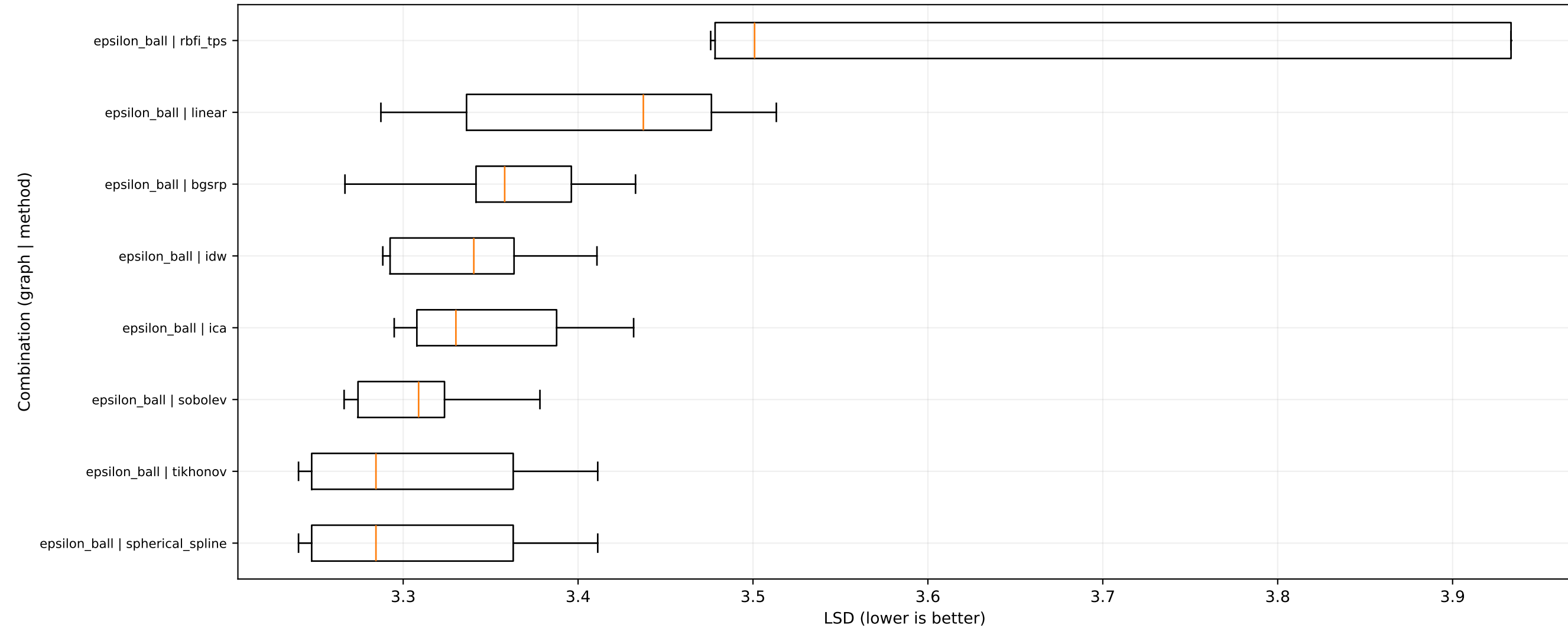
LSD distribution by graph-method combination - dataset: iris_graph_signal
