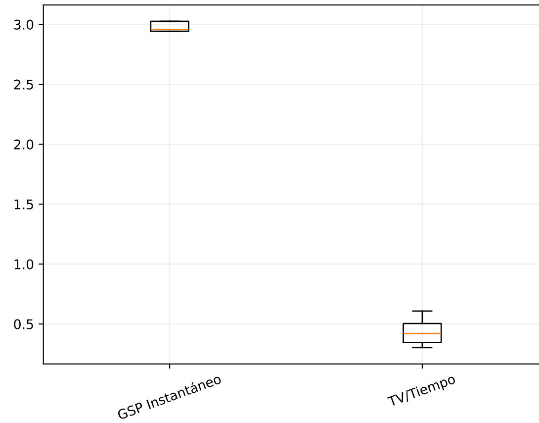
LSD
