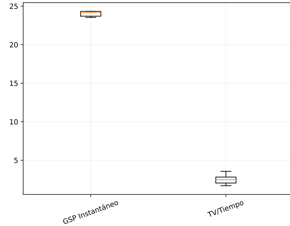
coherence_mean
