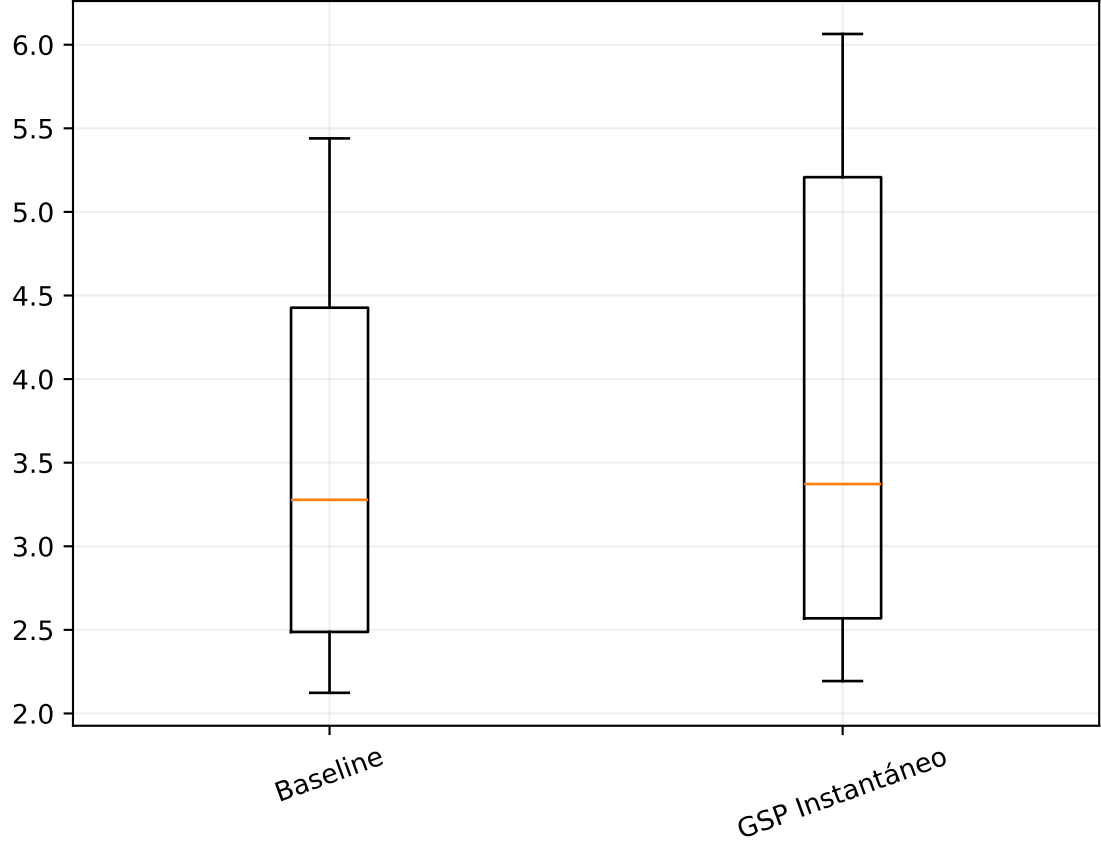
coherence_mean
