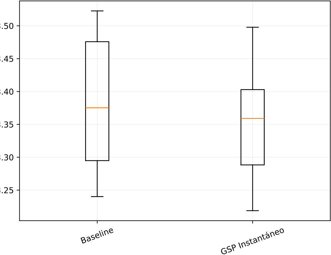
LSD
