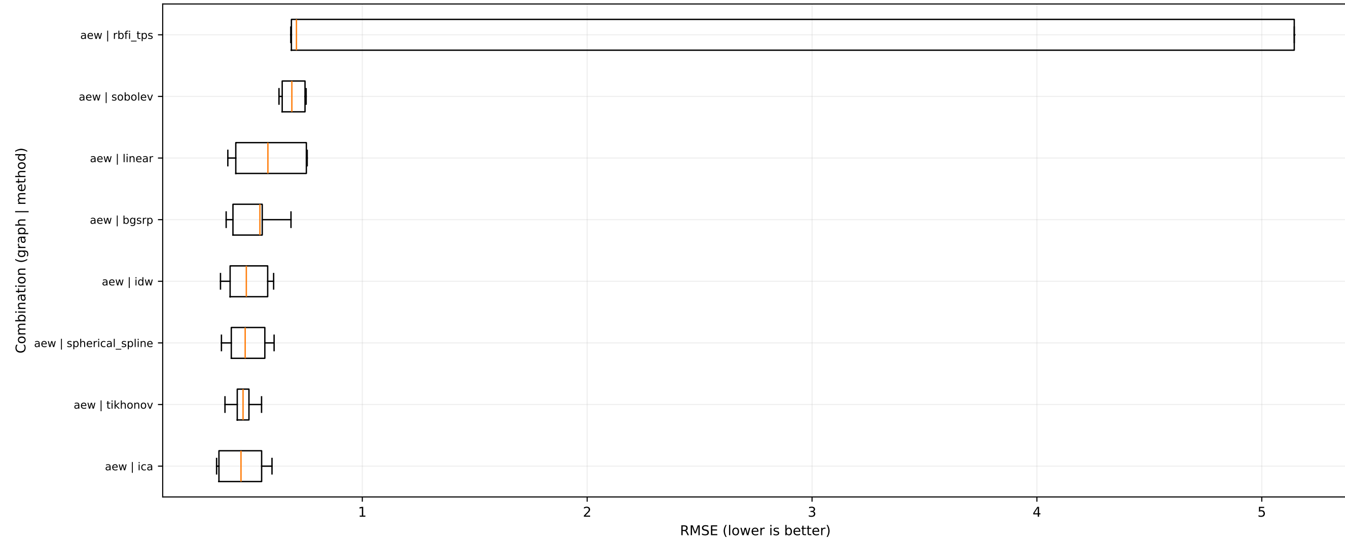
RMSE distribution by graph-method combination - dataset: iris_graph_signal
