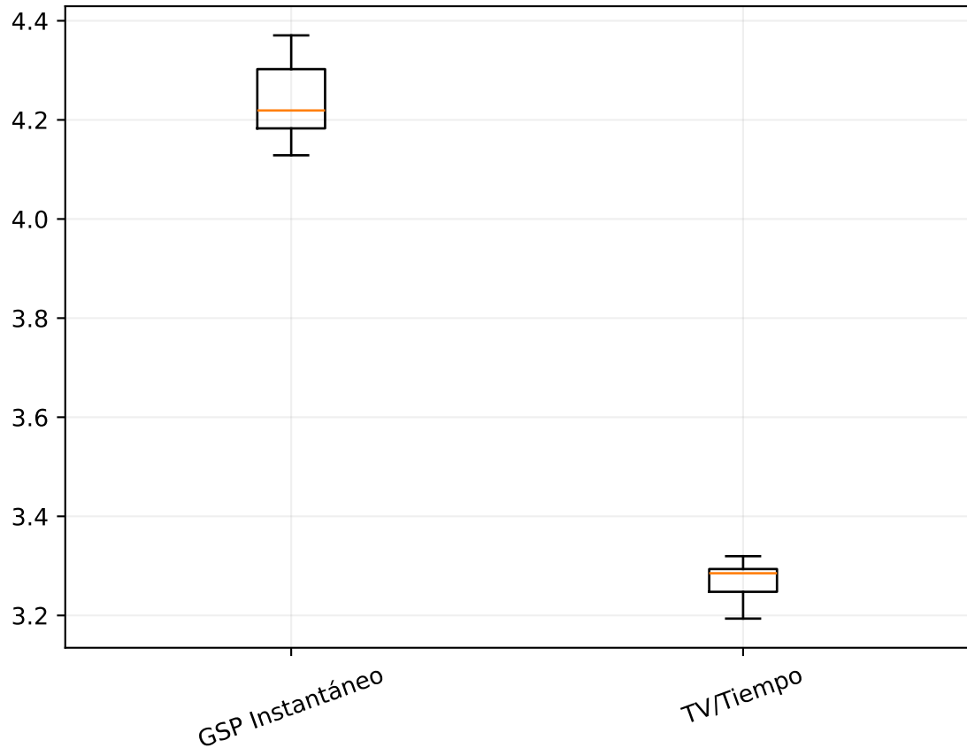
LSD
