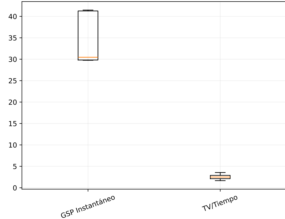
DTW
