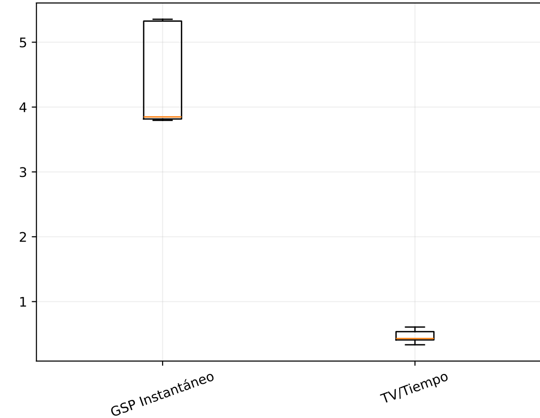
RMSE
