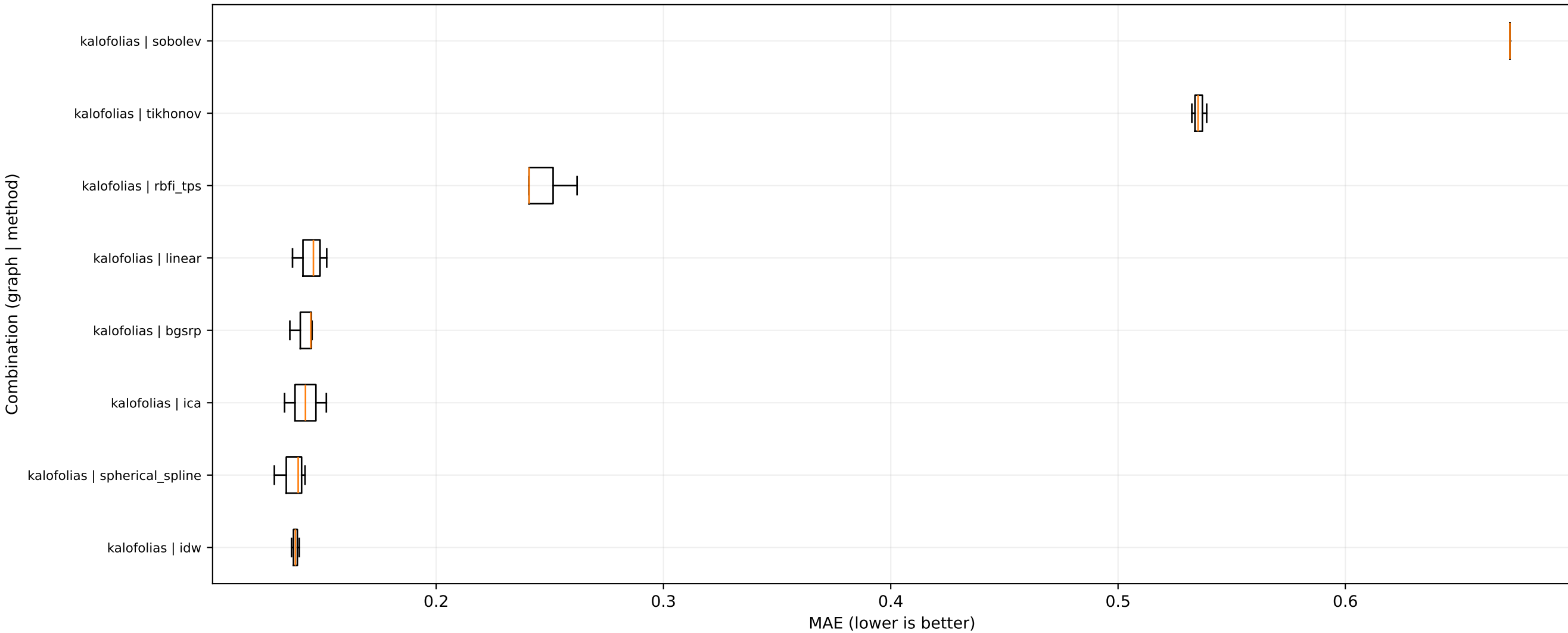
MAE distribution by graph-method combination - dataset: iris_graph_signal
