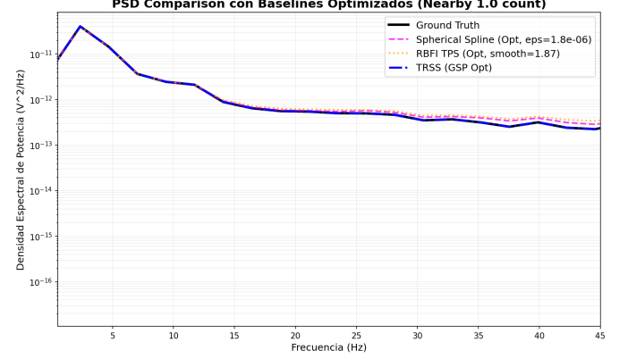
Fig. 5. Power Spectral Density (PSD) comparison. Temporal regularization accurately maintains the spectral power distribution across critical physiological bands (alpha, beta).
