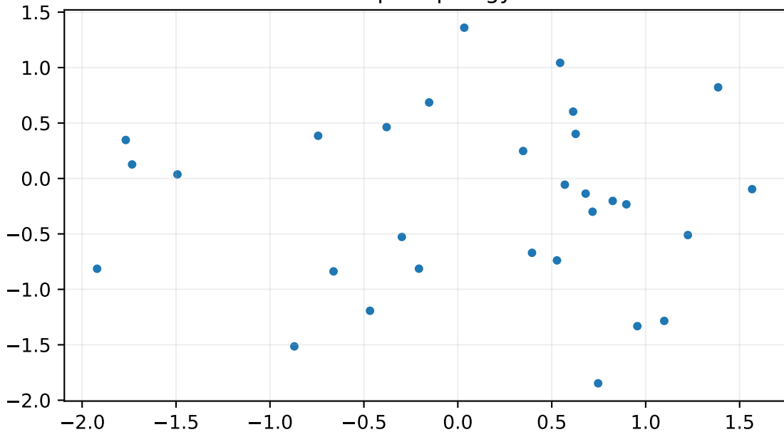
Graph topology
