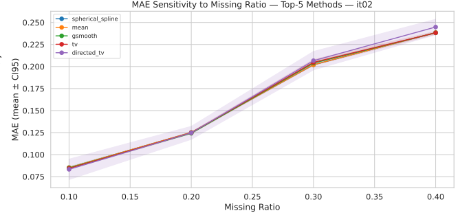
Fig. 2. MAE sensitivity to missing-channel ratio (top-5 methods), iteration it02 .
