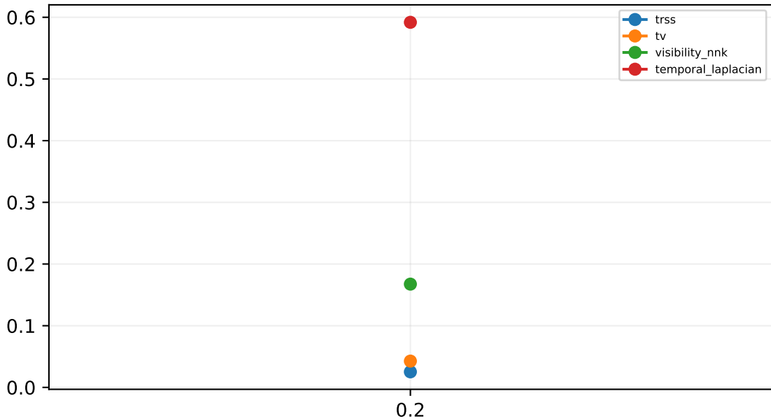
Scenario sensitivity
