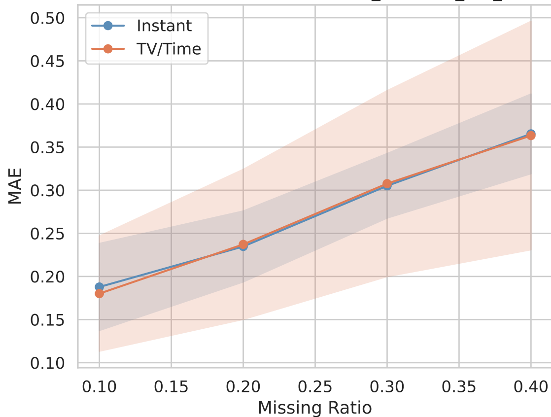
MAE — TV/Time vs Instant — it09_tikhonov_rbf_focus
