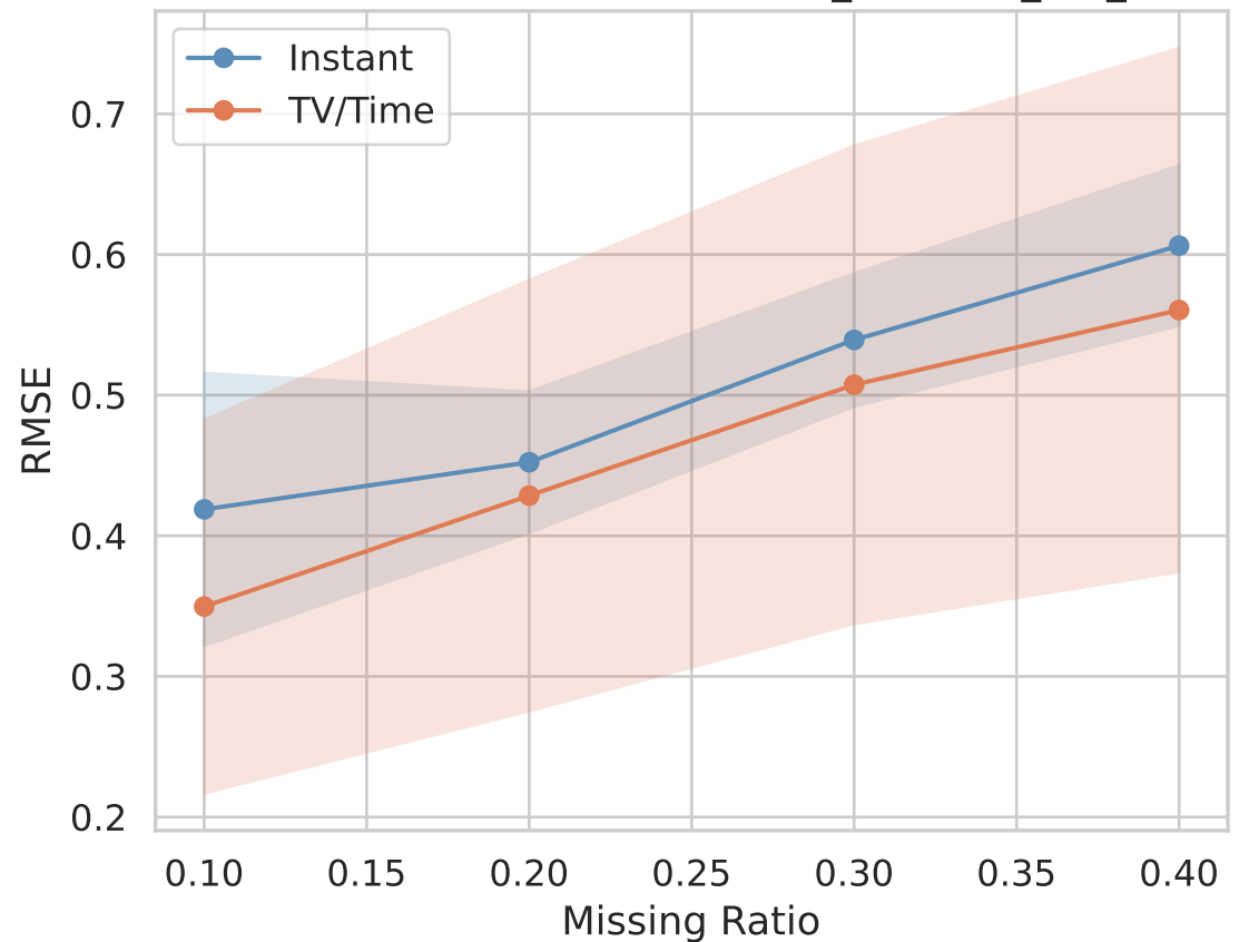
RMSE — TV/Time vs Instant — it09_tikhonov_rbf_focus
