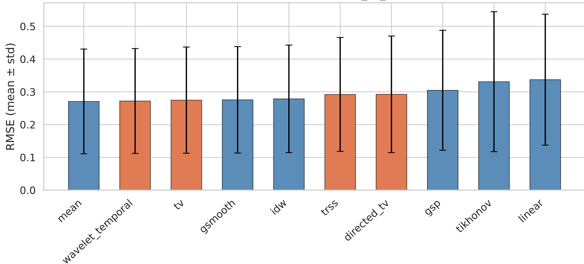
Top-10 Methods: RMSE — it05_all_datasets
