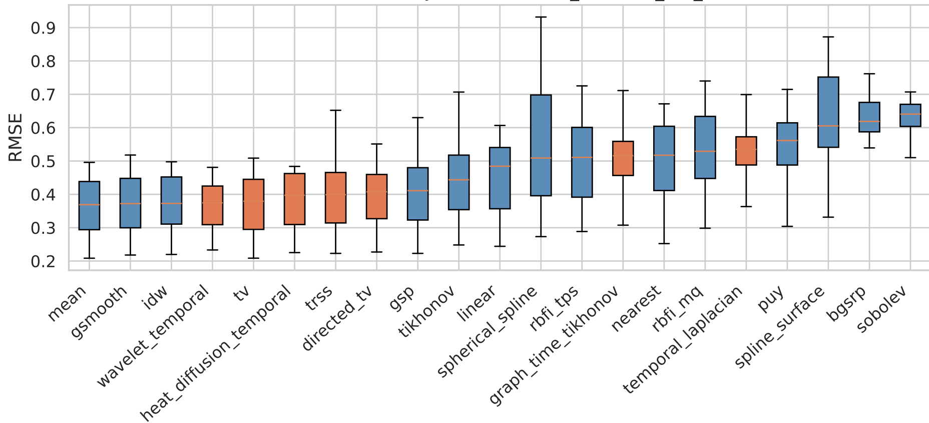
RMSE Distribution by Method — it09_tikhonov_rbf_focus
