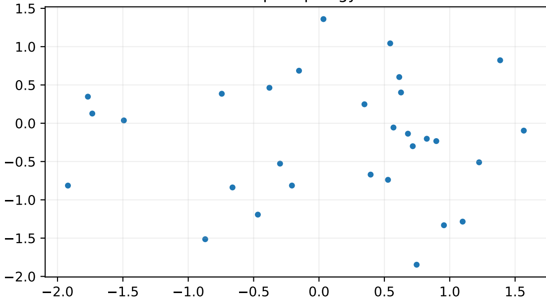
Graph topology
