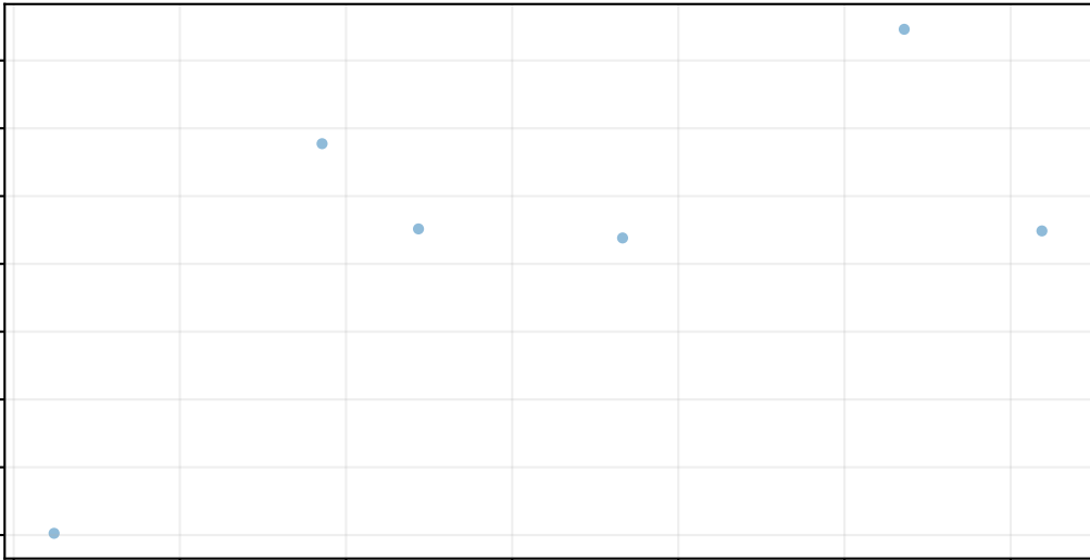
MAE vs RMSE
