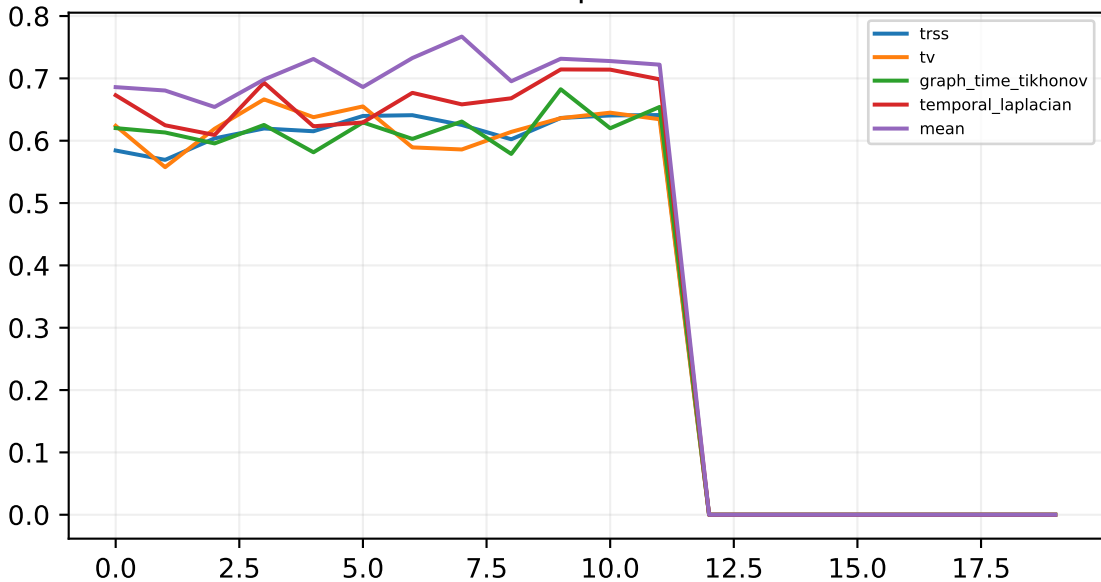
RMSE profiles
