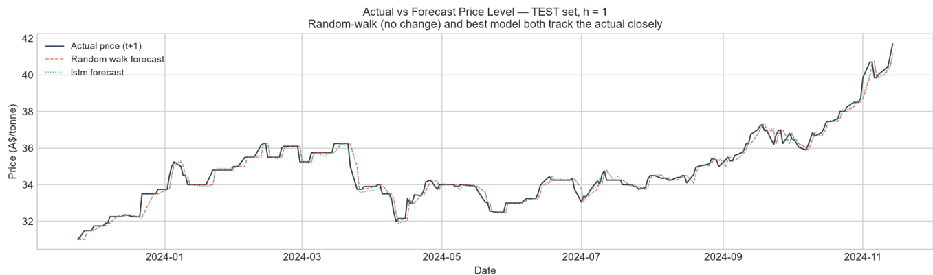
Figure 10. Actual next-day price level vs random-walk and best-model forecasts on the test set ( h = 1 ). The three lines nearly overlap, illustrating why marginal RMSE differences are statistically insignificant.
