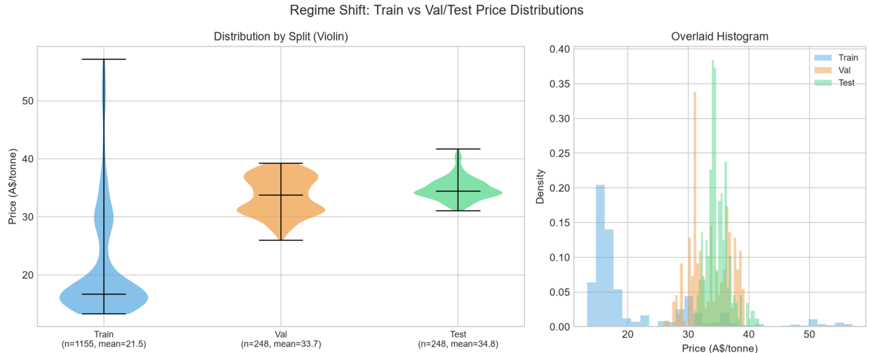
Figure 2. Price distribution by split (violin plot, left; overlaid histogram, right). The training distribution is wide and right-skewed due to the 2021-22 price spike pulling the upper tail; validation and test occupy a narrower high-price regime.
