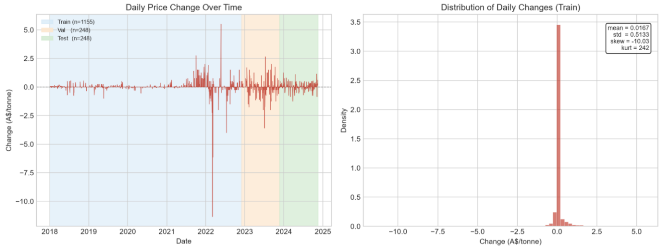
Figure 6. Daily price changes over the full sample period (left panel) and the distribution of daily changes on the training set (right panel). Near-zero mean; heavy tails; extreme excess kurtosis.
