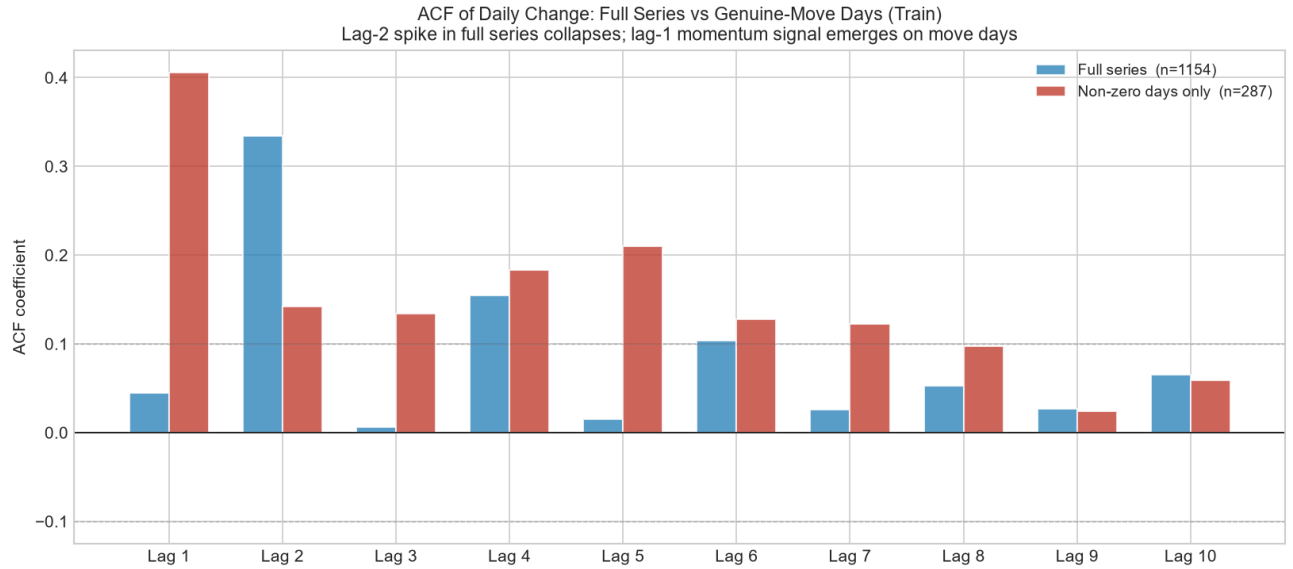
Figure 5. ACF of daily price change: full series (blue) vs genuine-move days only (red), training set. The lag-2 spike collapses from \approx 0.33 to \approx 0.14 — a forward-fill artefact. The lag-1 momentum signal ( \approx 0.41 ) on move-days is genuine.
