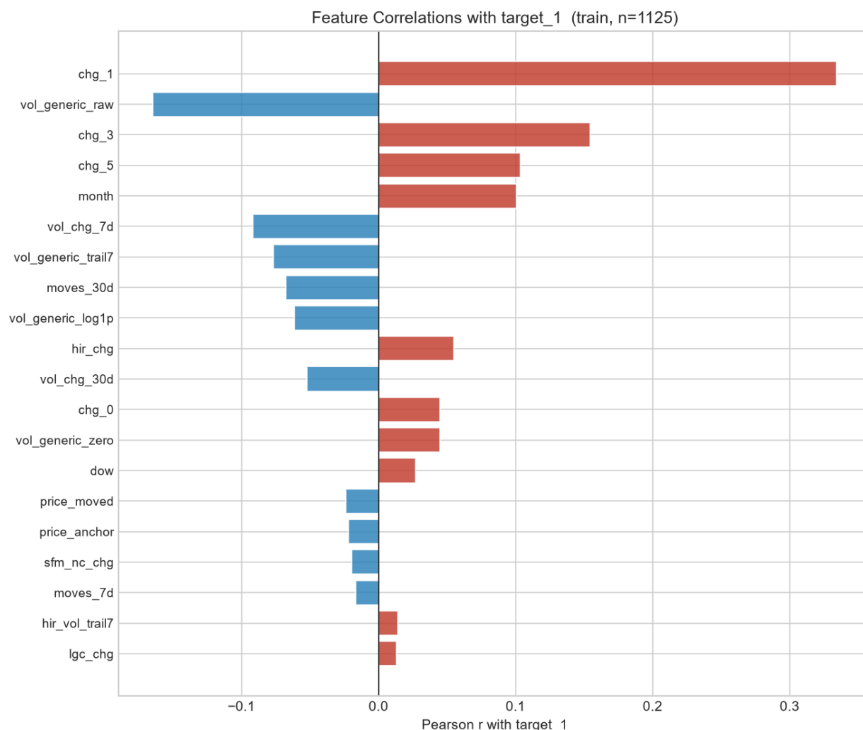
Figure 8. Pearson correlations of each feature with the 1-day-ahead target (target_1) on the training set. Positive (red) bars indicate momentum-aligned features; negative (blue) bars indicate mean-reverting signals. Lagged momentum changes (chg_1, chg_3, chg_5), volume metrics, and calendar features dominate the top correlation rankings.
