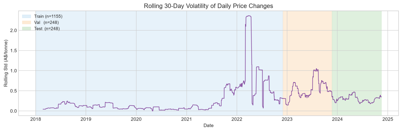
Figure 7. Rolling 30-day standard deviation of daily price changes. Volatility clustering is visible: the 2021-22 spike period shows markedly higher volatility than the surrounding years.
