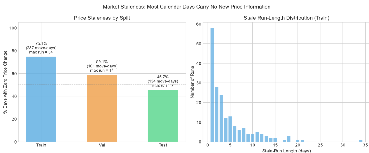
Figure 3. Left: percentage of zero-change days by split (with number of genuine move-days and longest stale run annotated). Right: distribution of stale run lengths in the training set — runs of 5 or more consecutive stale days are common, with a maximum run exceeding 30 days.
