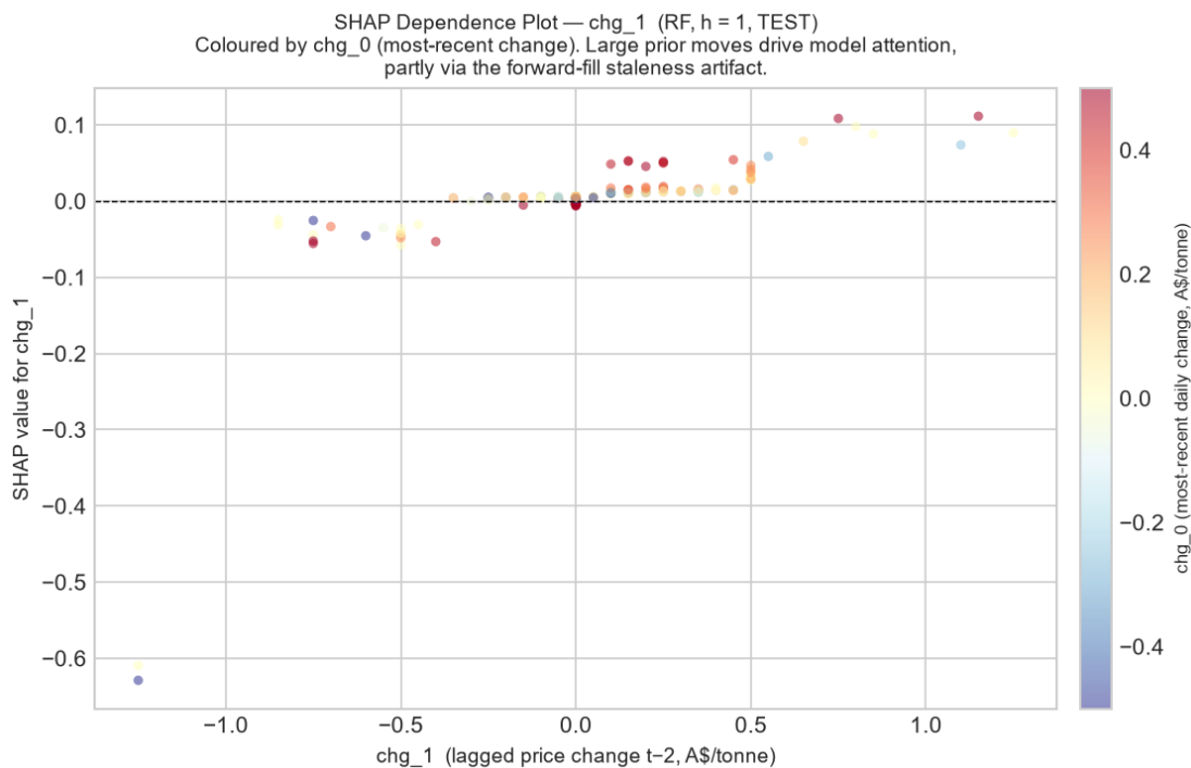
Figure 13. SHAP dependence plot for chg_1 (change at t-2 ), h = 1 , test set. Each point is one test observation; colour = chg_0 (most-recent change). The pattern shows that large prior moves raise the model's attention — partly a genuine staleness regime
