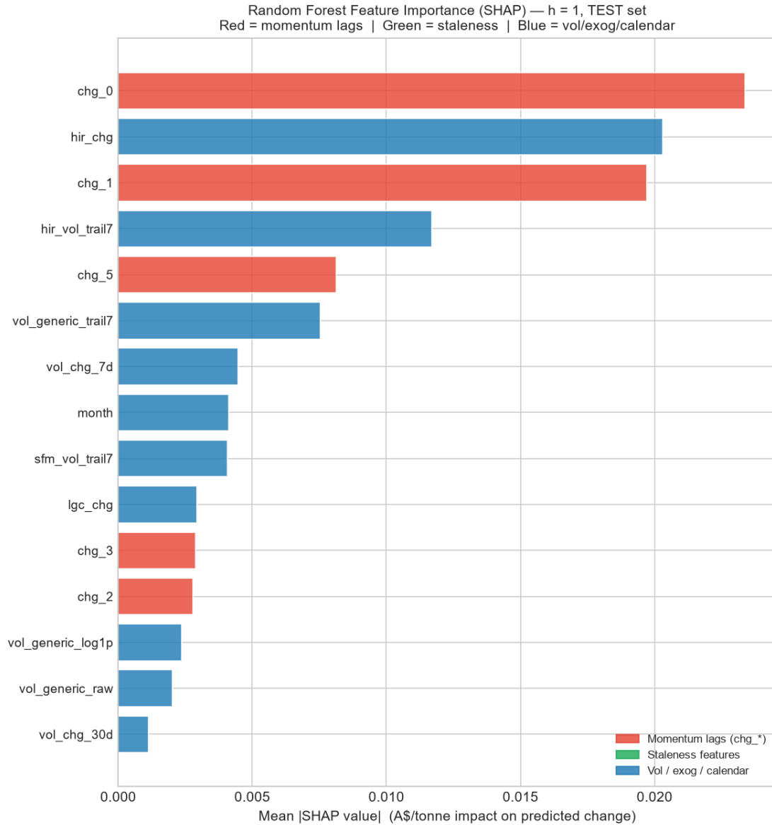
Figure 12. Feature importance for Random Forest ( h = 1 , test set) ranked by mean |SHAP| value. Red bars = momentum lag features ( chg_* ); green = staleness features; blue = volatility, volume, exogenous, calendar. The dominant drivers are chg_0 (recent momentum) and hir\_chg (HIR cross-market change), with volume/volatility metrics in the mid-range. No staleness feature appears in the top 8.
