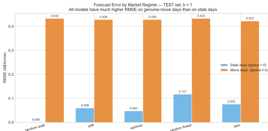
Figure 11. RMSE decomposed into stale days (actual price change = 0) and genuine-move days (actual price change \neq 0 ), h = 1 , test set. All models achieve near-zero RMSE on stale days (trivially correct) but have substantially higher errors on move days, confirming that the genuine forecasting challenge lies in predicting when and by how much prices move.
