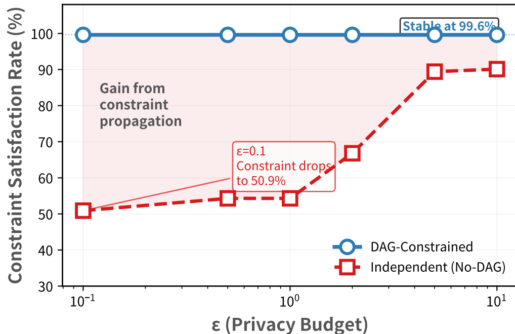
DAG Constraint Preservation
