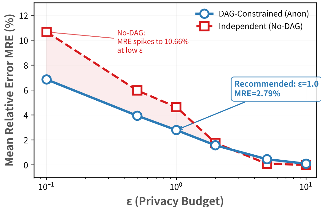
T2 Numerical Perturbation Accuracy
