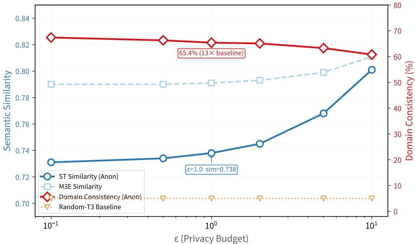
T3 Medical Semantic Perturbation: Privacy-Utility Tradeoff
