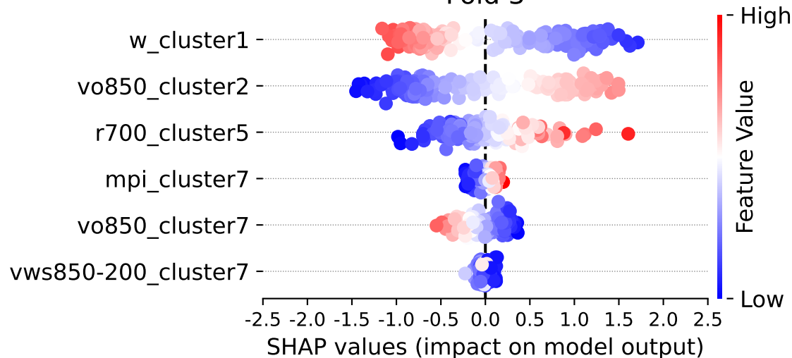
Fold 3
