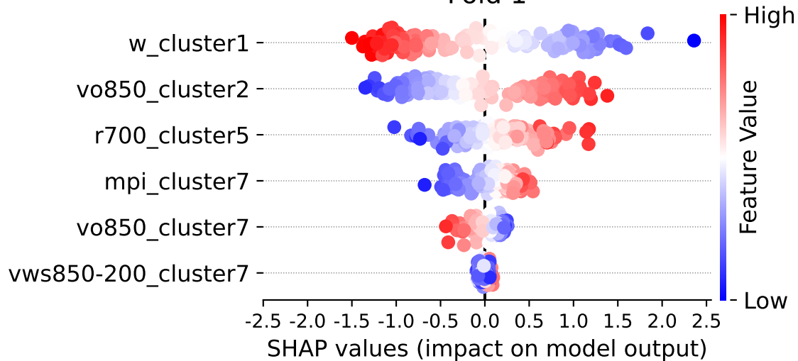
Fold 1
