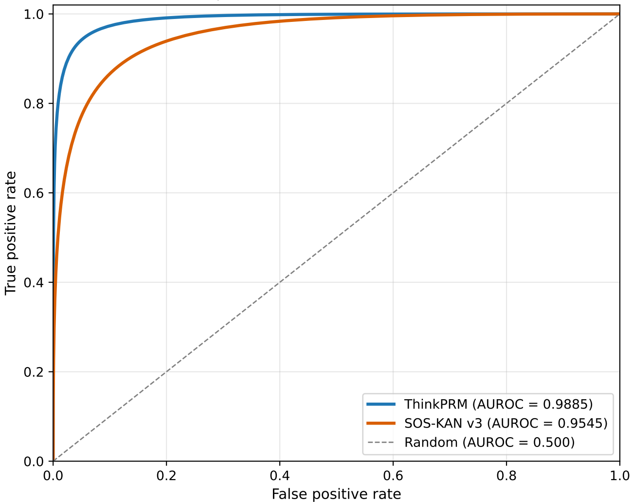
Figure 2 - ROC curves on FoVer corpus (6,548 pairs) Curves illustrate published AUROC; binormal-fit, not a re-evaluation
