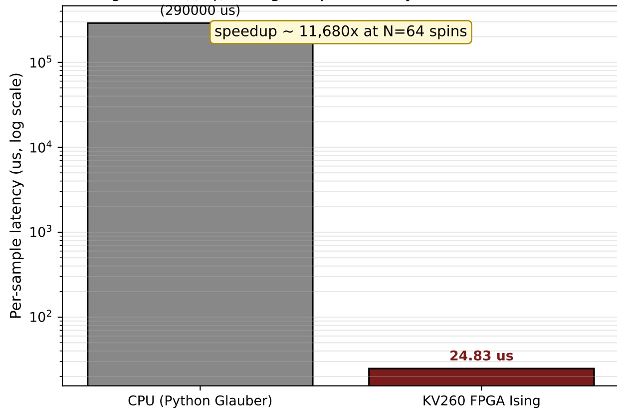
Figure 3 - 64 spin Ising-sampler latency: CPU vs KV260 FPGA
