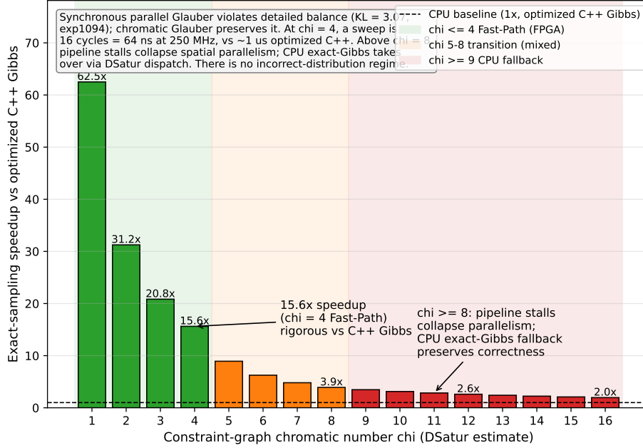
Figure 7 - \chi \leq 4 Sparse-Constraint Accelerator: speedup is a step function of constraint topology. KL = 3.07 forced this architecture.
