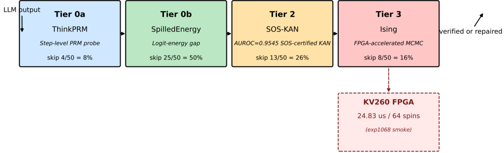
Figure 1: Carnot 4-tier verification cascade with empirical skip-tier rates from exp1073 (n=50). Tier 0a ThinkPRM, Tier 0b SpilledEnergy, Tier 2 SOS-KAN, Tier 3 Ising MCMC with KV260 FPGA acceleration callout.
