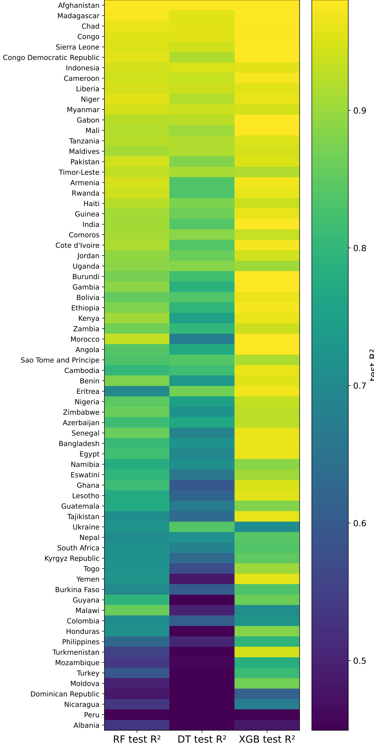
Per-country predictive performance (test R 2 ) — sorted by mean performance
