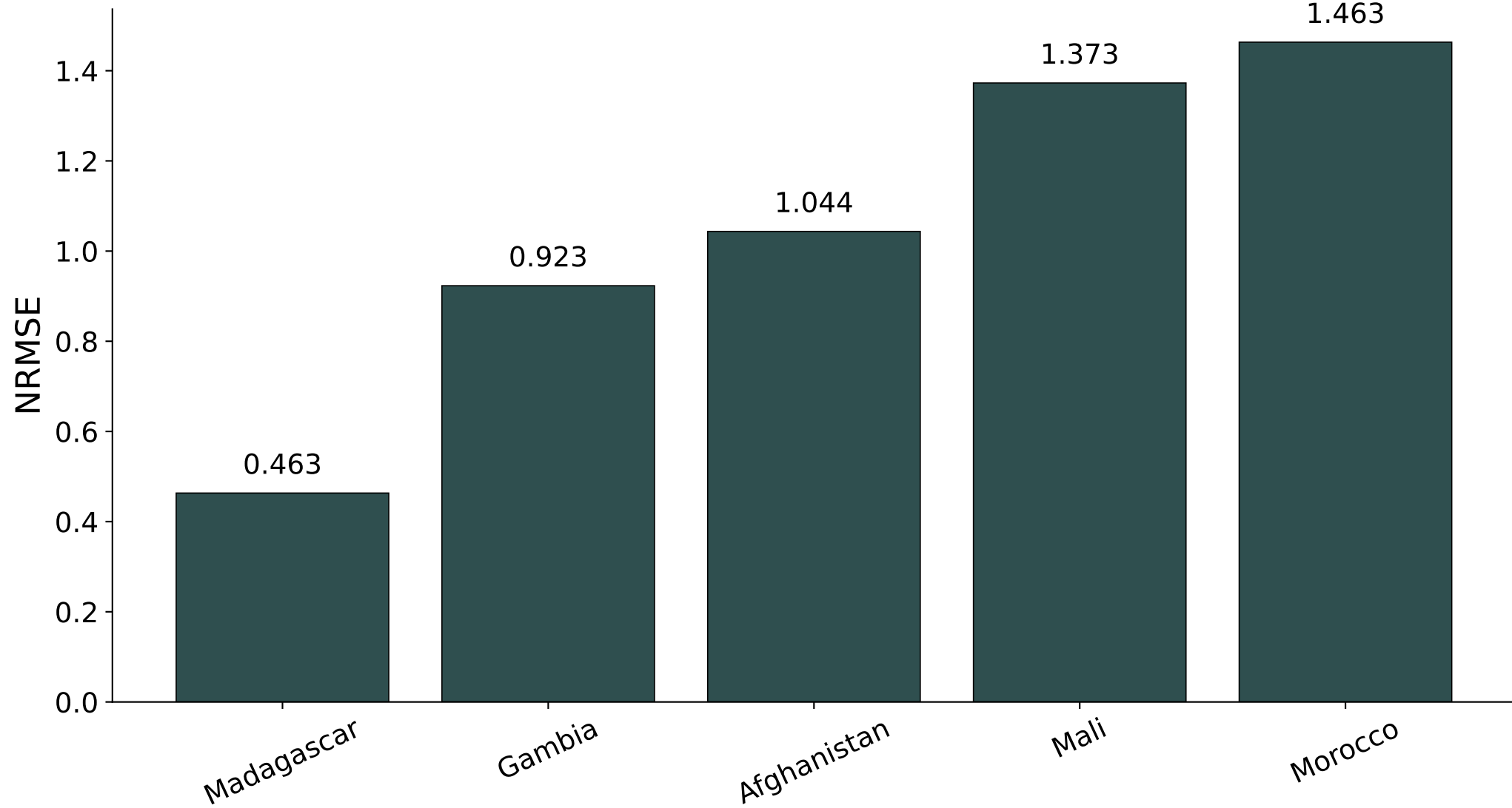
Top-5 countries — XGBoost normalized RMSE
