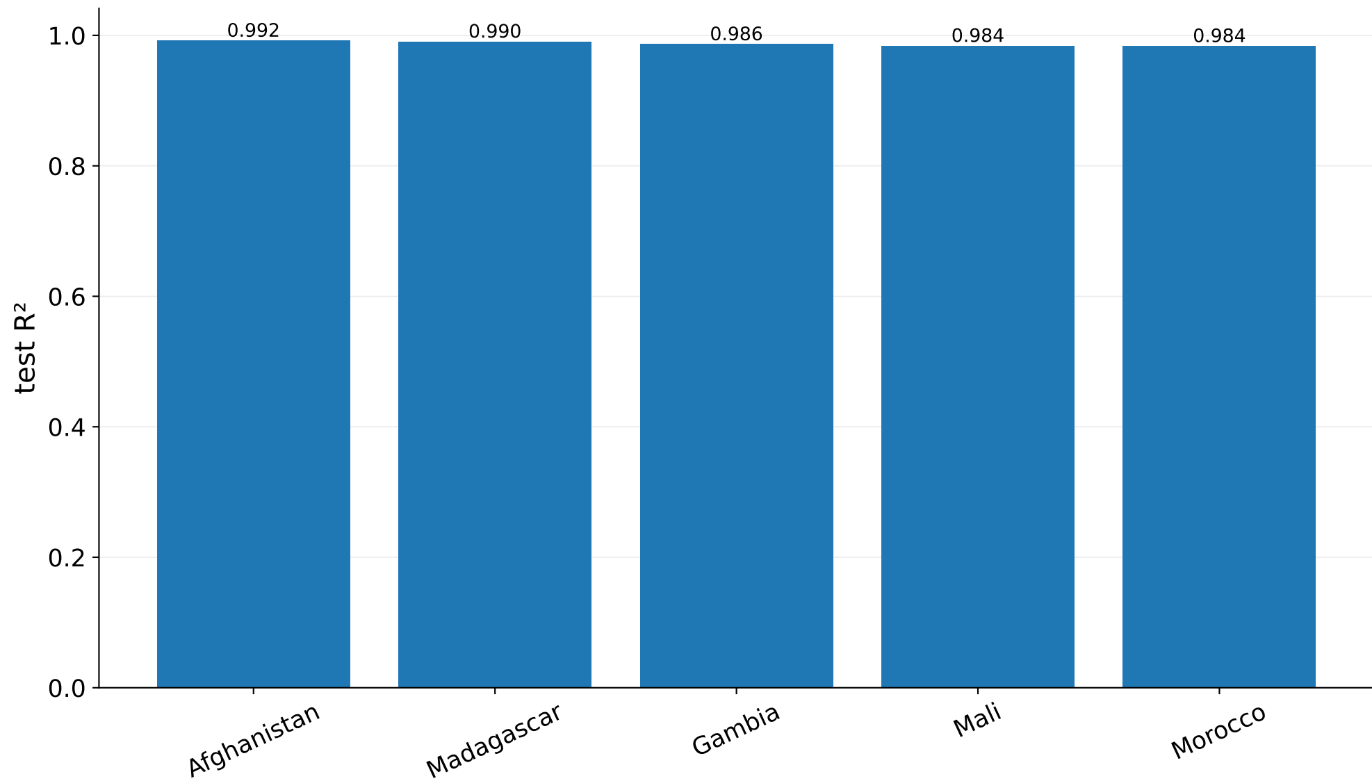
Top-5 countries by XGBoost performance (test R^2 )
