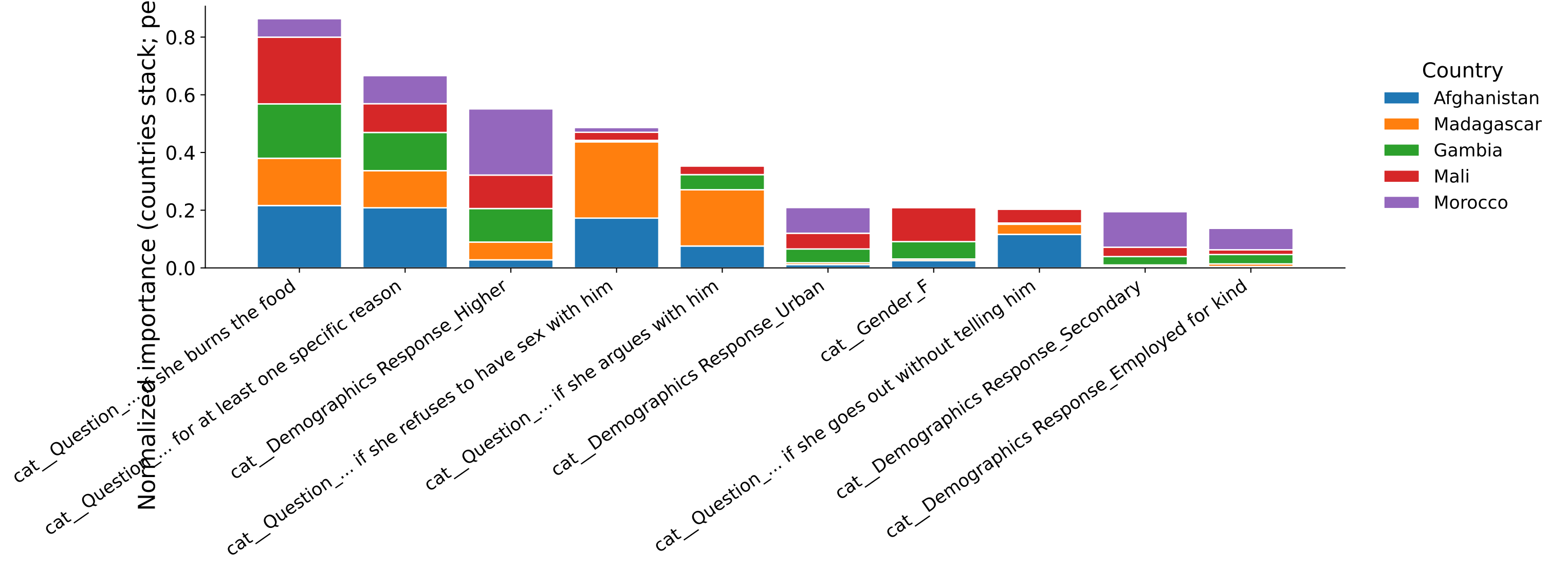
Top-5 countries by XGBoost test R 2 — feature importance (features on x-axis; colors = countries)
