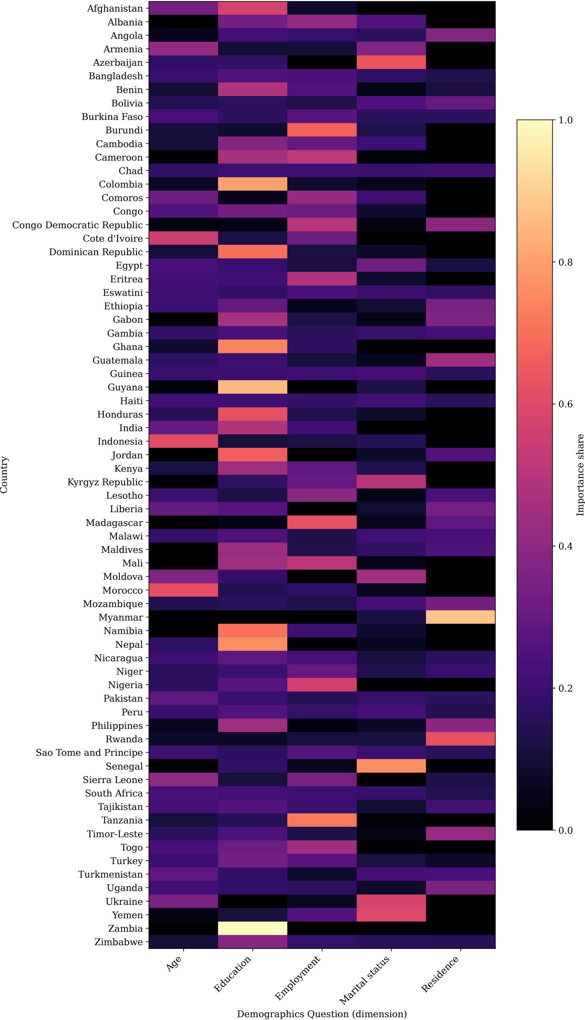
Part II — Importance share by demographic dimension (XGBoost, demographics-only)
