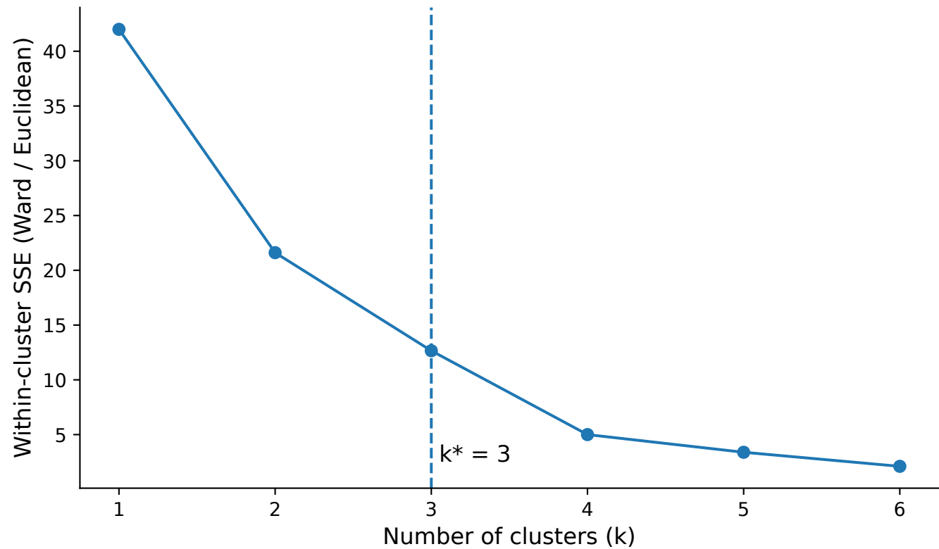
Elbow curve (selected countries)
