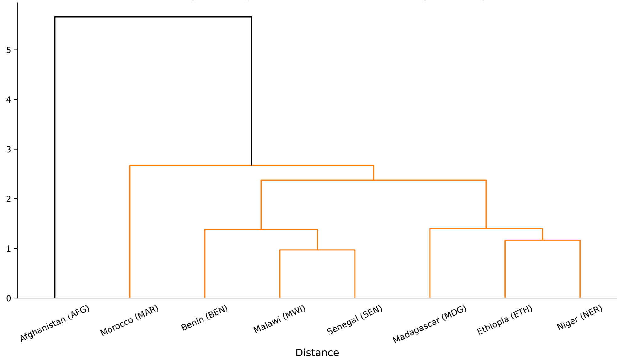
P1/P2-only dendrogram (metric=euclidean, linkage=average)
