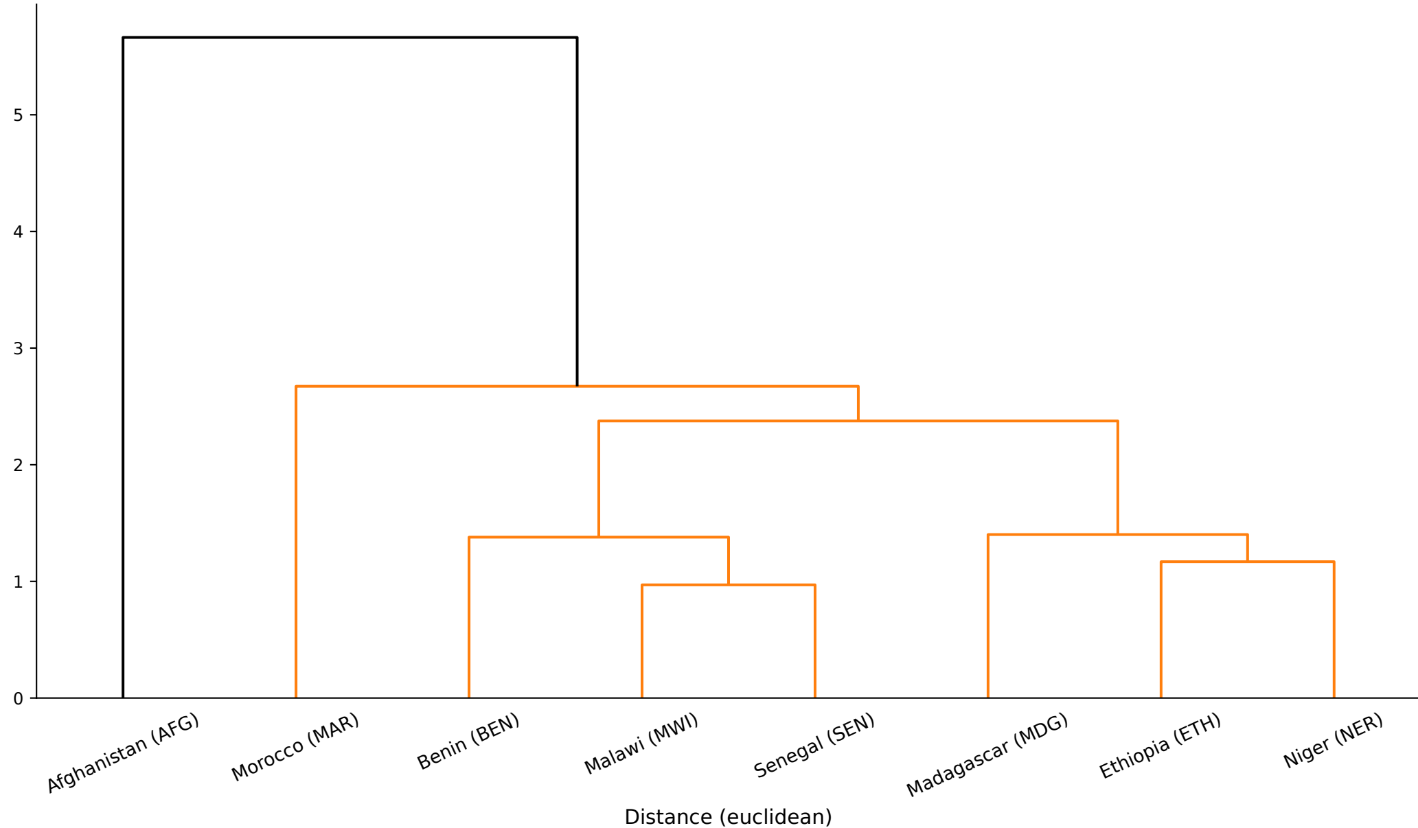
P1/P2-only country dendrogram (best: distance=euclidean, linkage=average)
