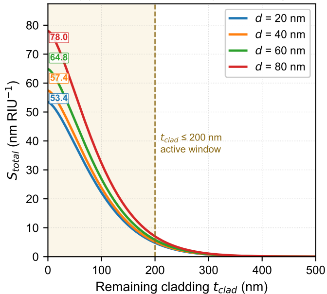
(b) Composite sensitivity vs cladding
