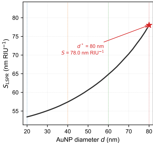
(a) LSPR sensitivity vs diameter
