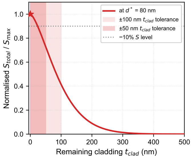
(b) Etch-depth tolerance (optimum: t_{clad} = 0 nm)
