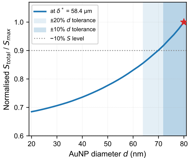
(a) Diameter tolerance (optimum: d^* = 80 nm)
