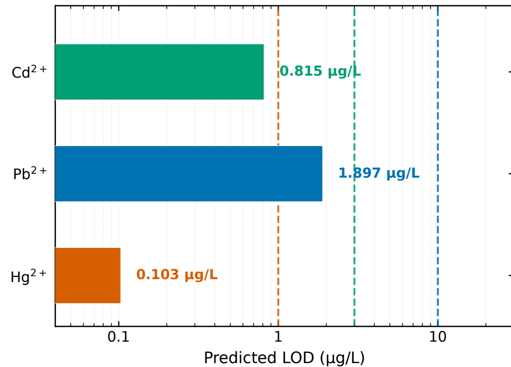
(a) Predicted LOD vs WHO guidelines ( S_{\text{total}} = 78.02 \text{ nm/RIU} )
