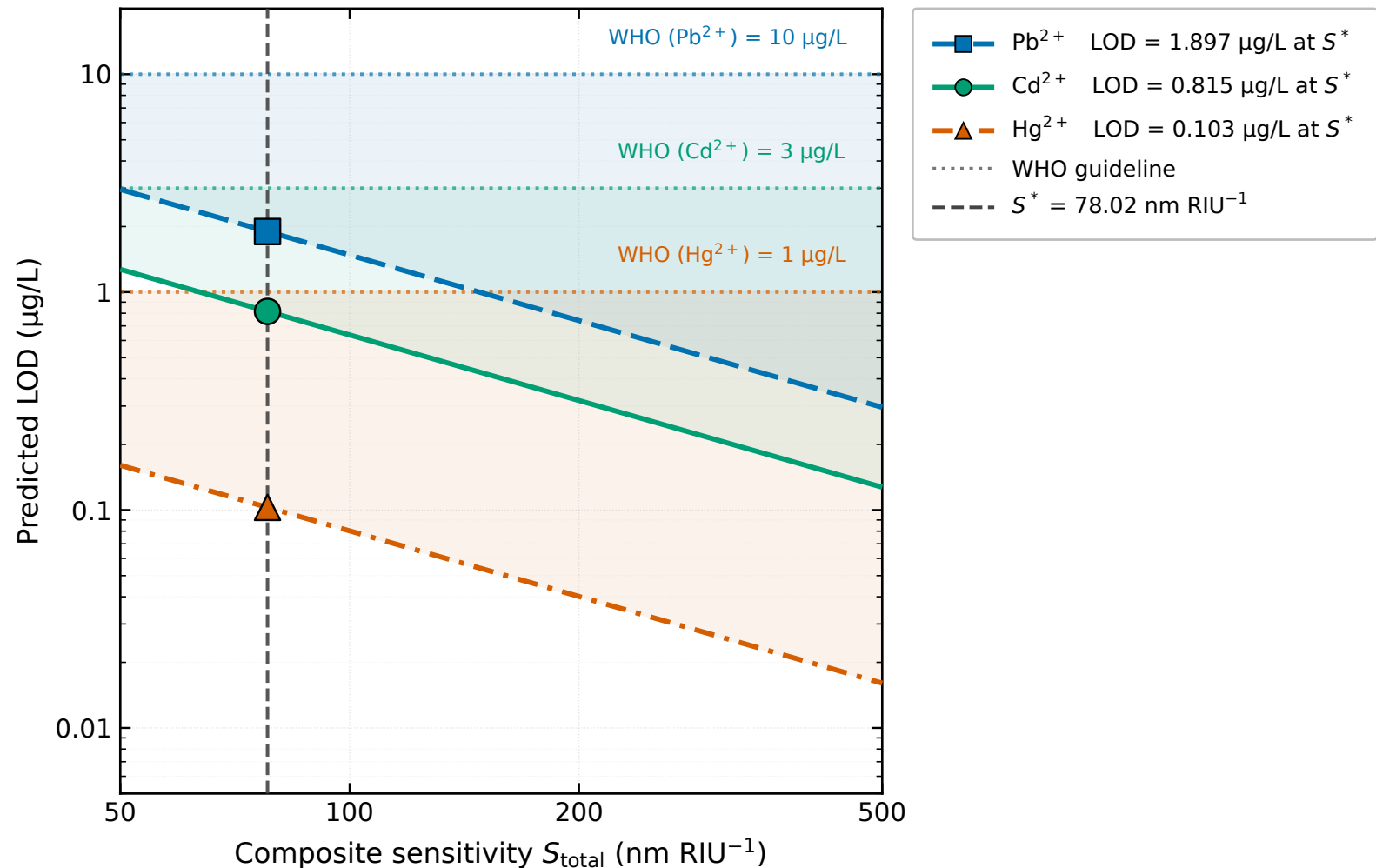
Sensitivity-LOD tradeoff for heavy metal detection
