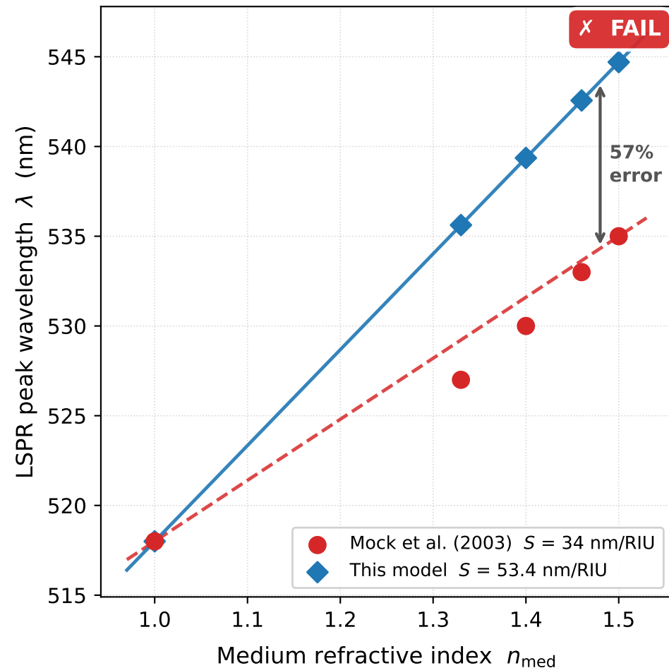
(b) LSPR bulk RI sensitivity — Mock et al. (2003)
