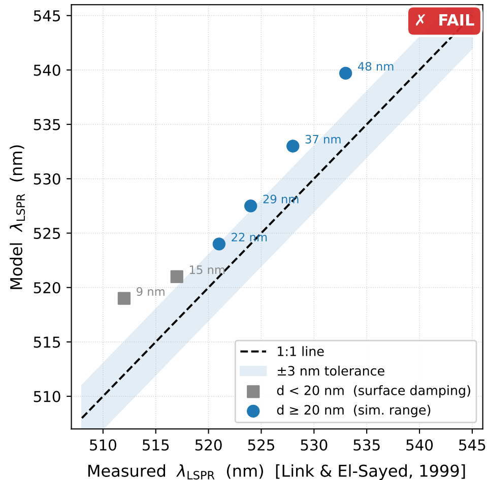
(a) Mie peak wavelength — Link & El-Sayed (1999)
