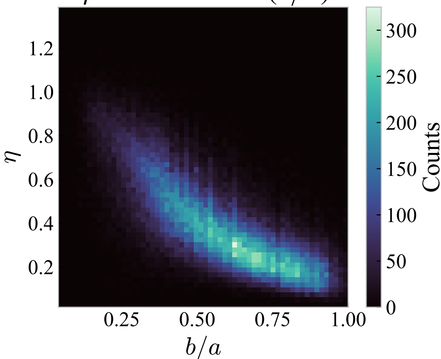
ination: Algorithm vs B/A ( q_0 = 0.20 )
