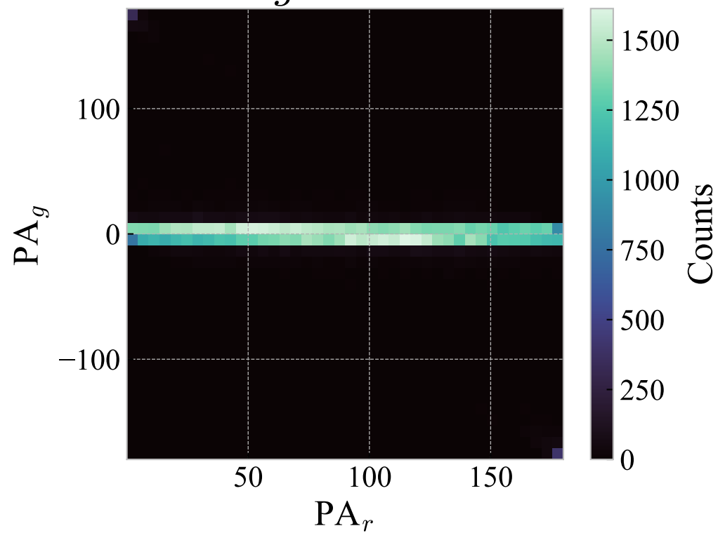
PA: g vs r Bands
