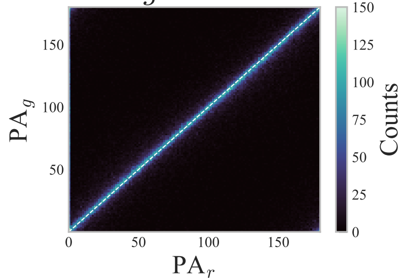
PA: g vs r Bands
