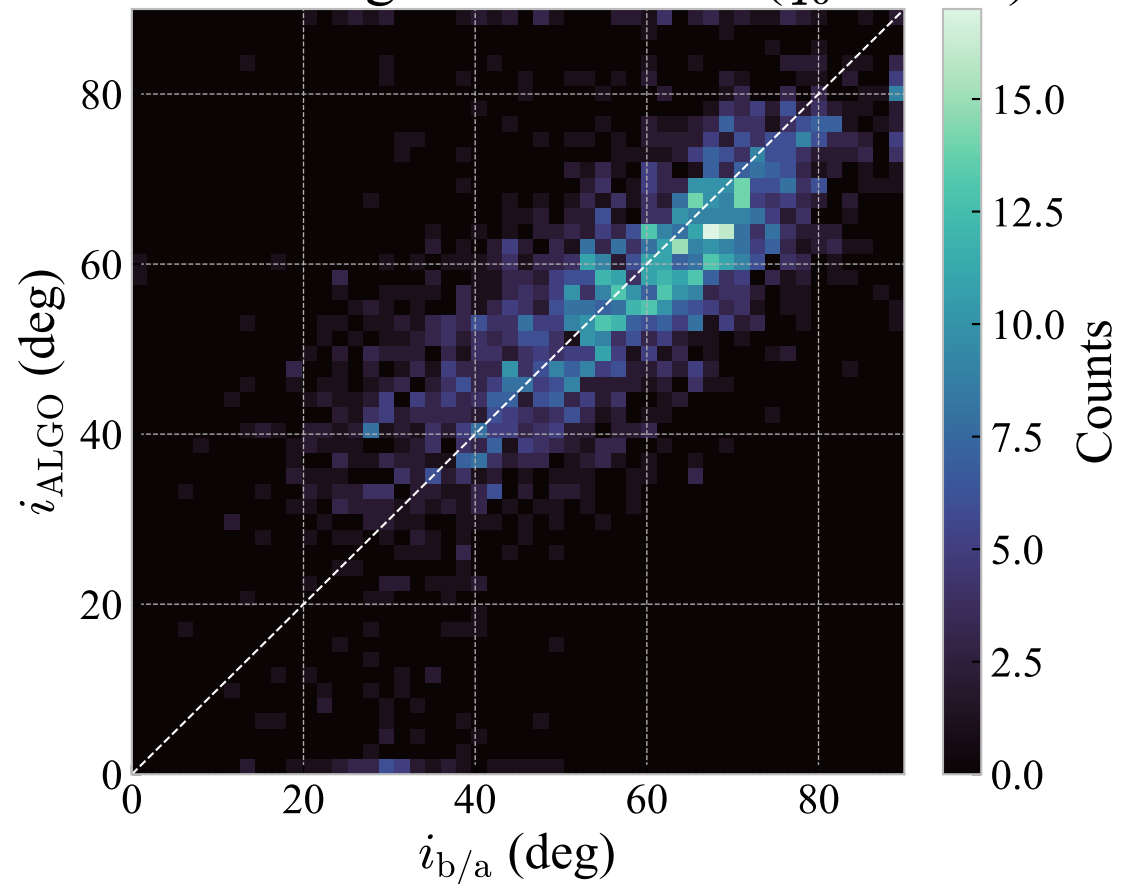
Inclination: Algorithm vs B/A ( q_0 = 0.20 )
