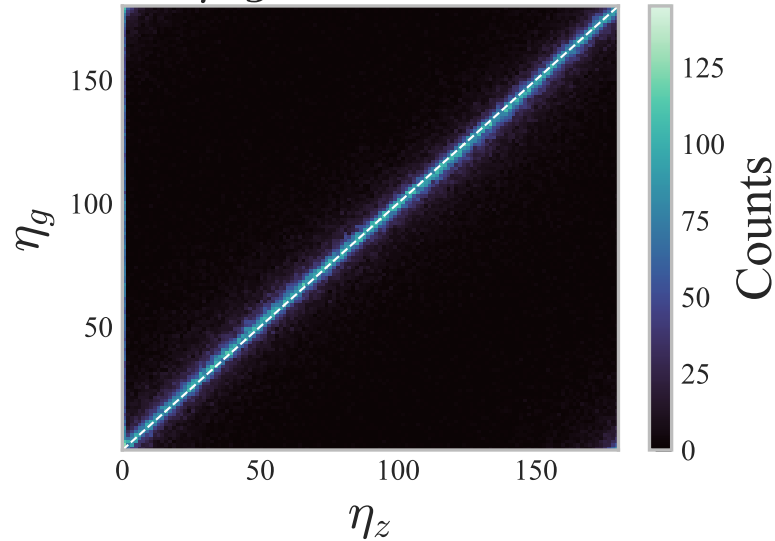
\eta : g vs z Bands
