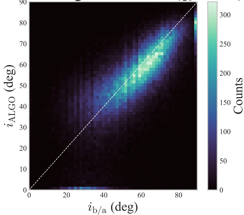
Inclination: Algorithm vs B/A ( q_0 = 0.20 )
