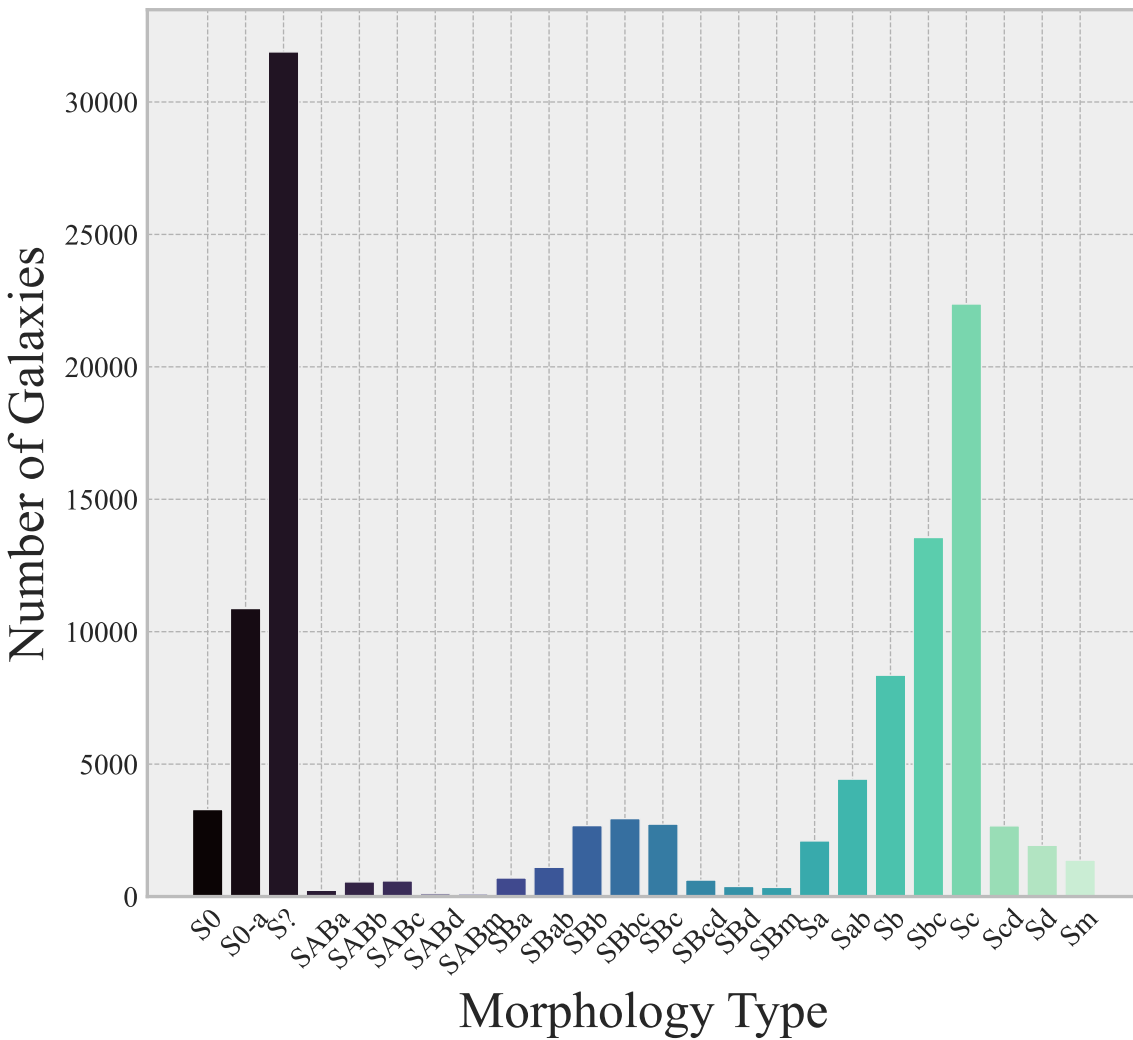
Full Dataset
