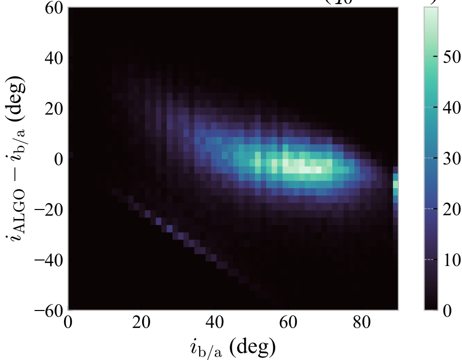
Difference B/A Inclination ( q_0 = 0.20 )
