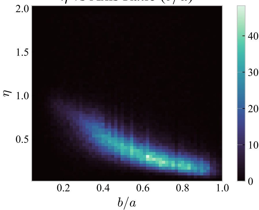
\eta vs Axis Ratio ( b/a )
