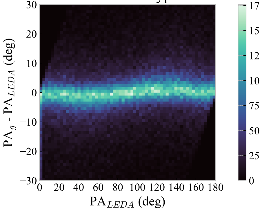
PA: Difference vs HyperLEDA
