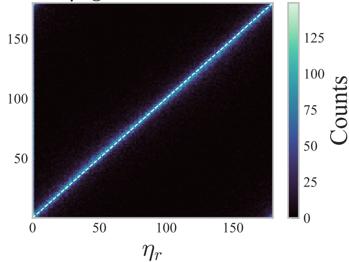
\eta : g vs r Bands
