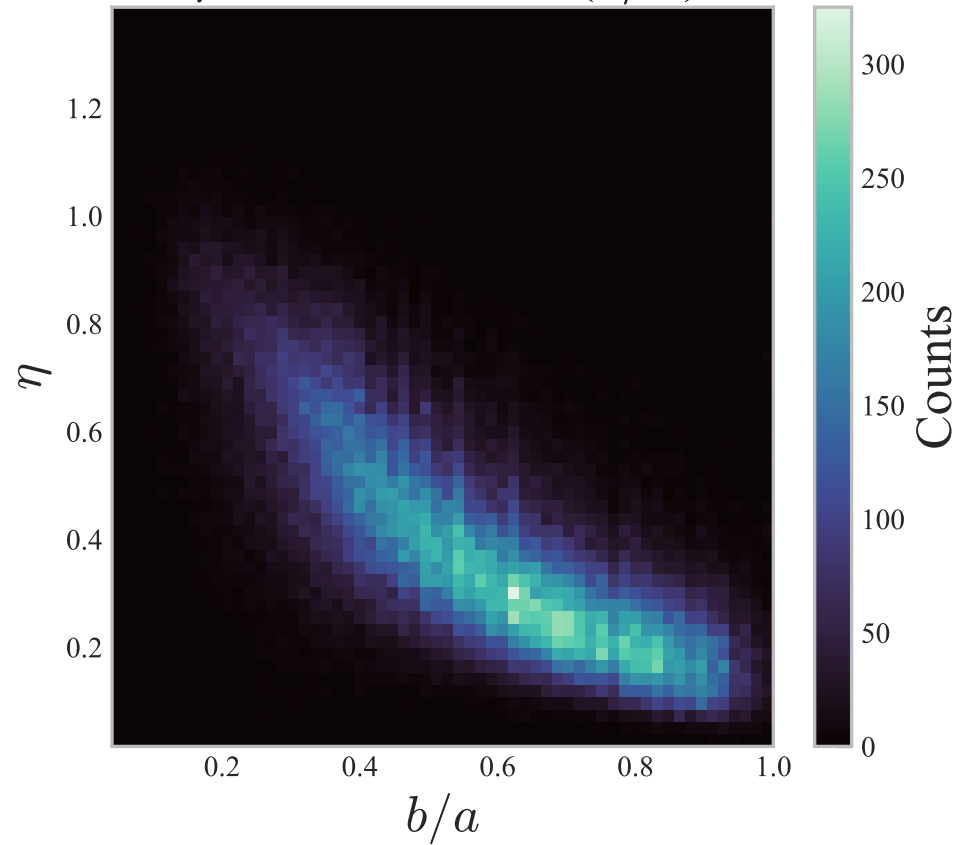
\eta vs Axis Ratio ( b/a )
