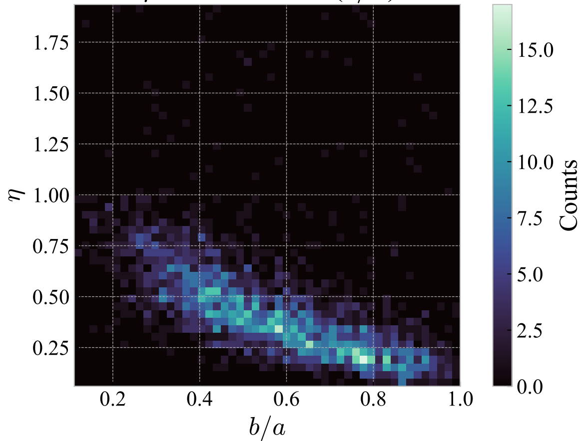
\eta vs Axis Ratio ( b/a )
