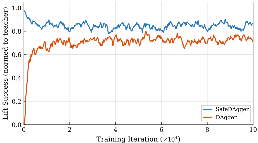
Student Policy Lift Success
