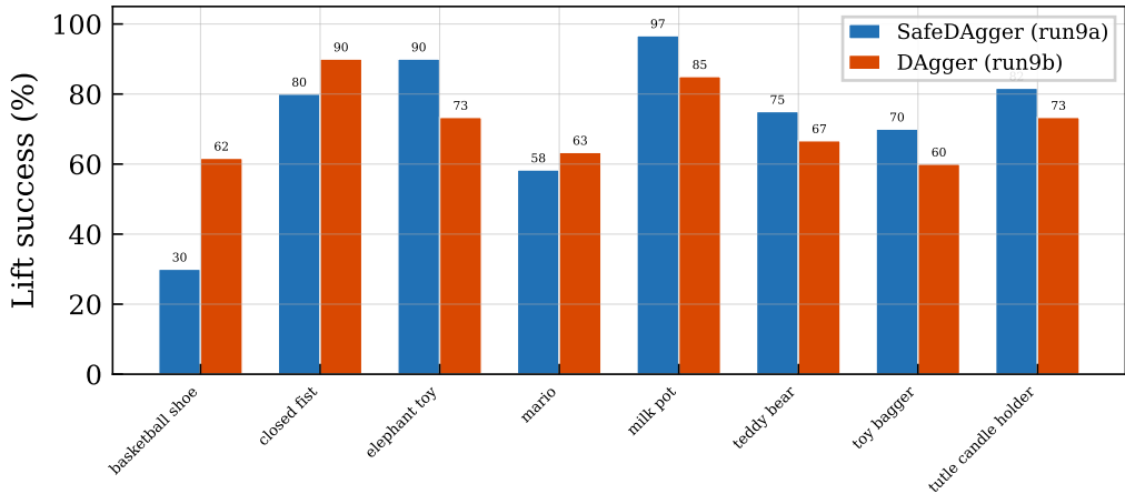
Per-Object Lift Success — Eval
