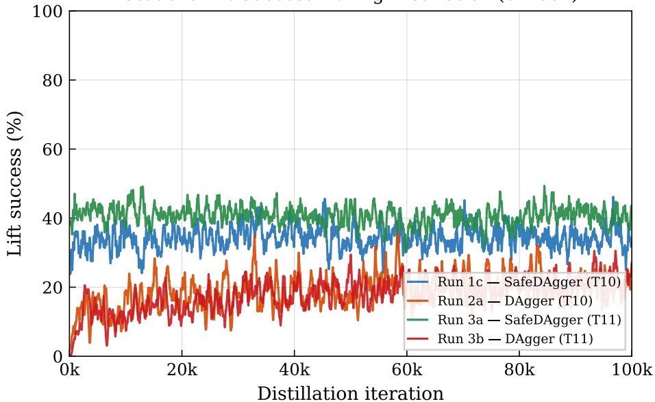
Student Lift Success During Distillation (0-100k)
